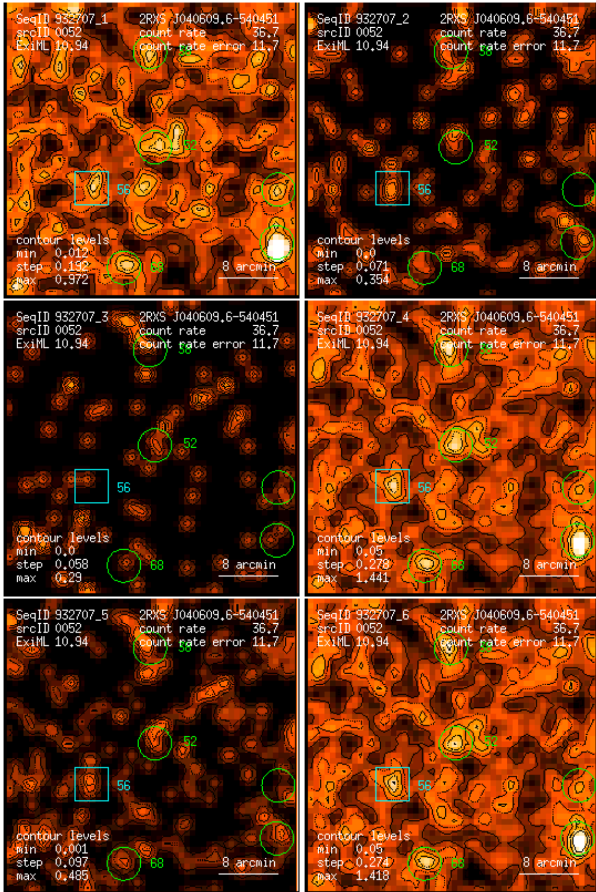
Figure 52: RASS 932707: detection 0052: band rate images, Gaussian filter: (1) PSPC channels 11 – 41, (2) 52 – 90, (3) 91 – 201, (4) 11 – 235, (5) 52 – 201, (6) 11 – 201. Broad band rates in counts/ks. Band rate contour levels in counts/ks/arcmin 2 .
