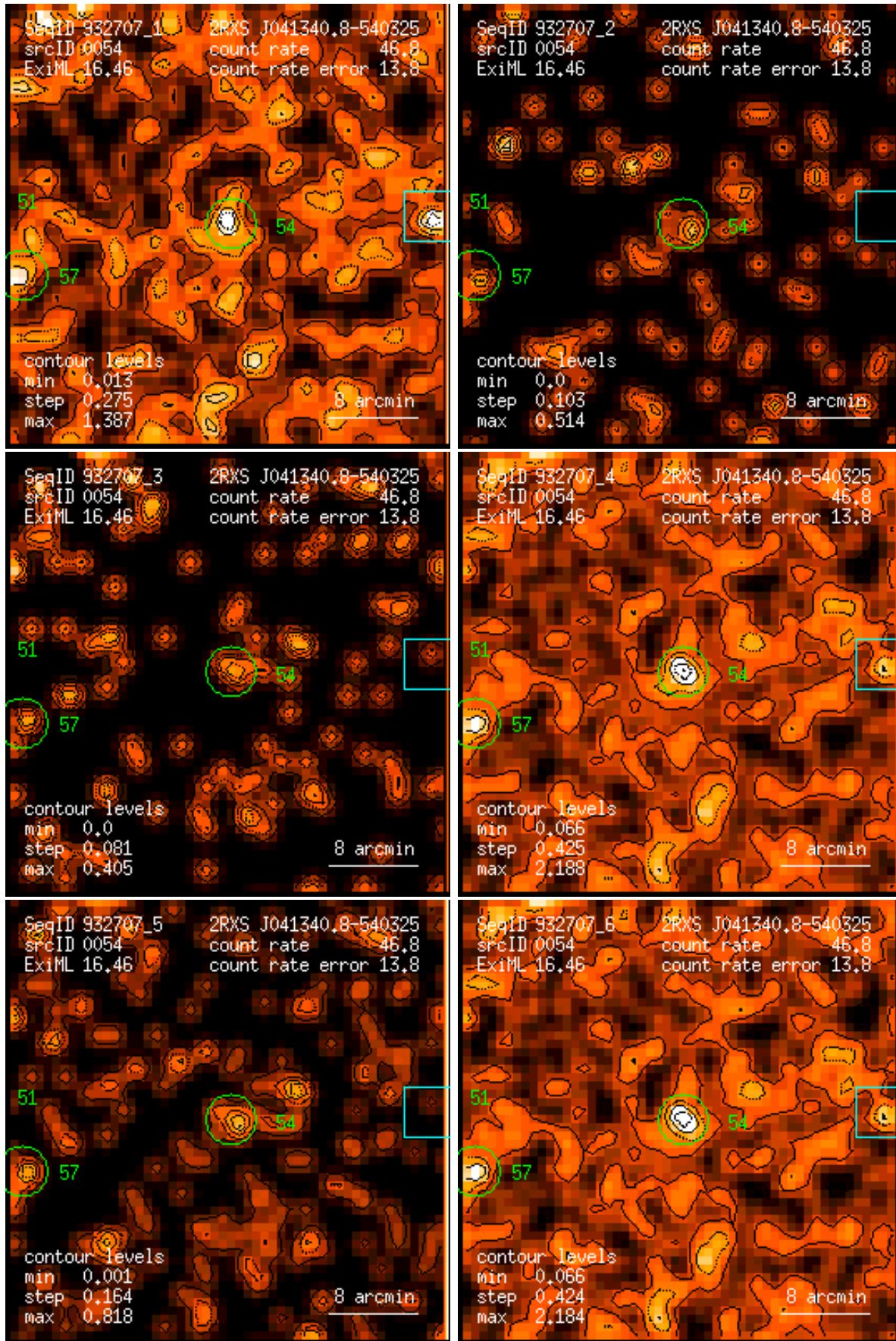
Figure 54: RASS 932707: detection 0054: band rate images, Gaussian filter: (1) PSPC channels 11 – 41, (2) 52 – 90, (3) 91 – 201, (4) 11 – 235, (5) 52 – 201, (6) 11 – 201. Broad band rates in counts/ks. Band rate contour levels in counts/ks/arcmin 2 .
