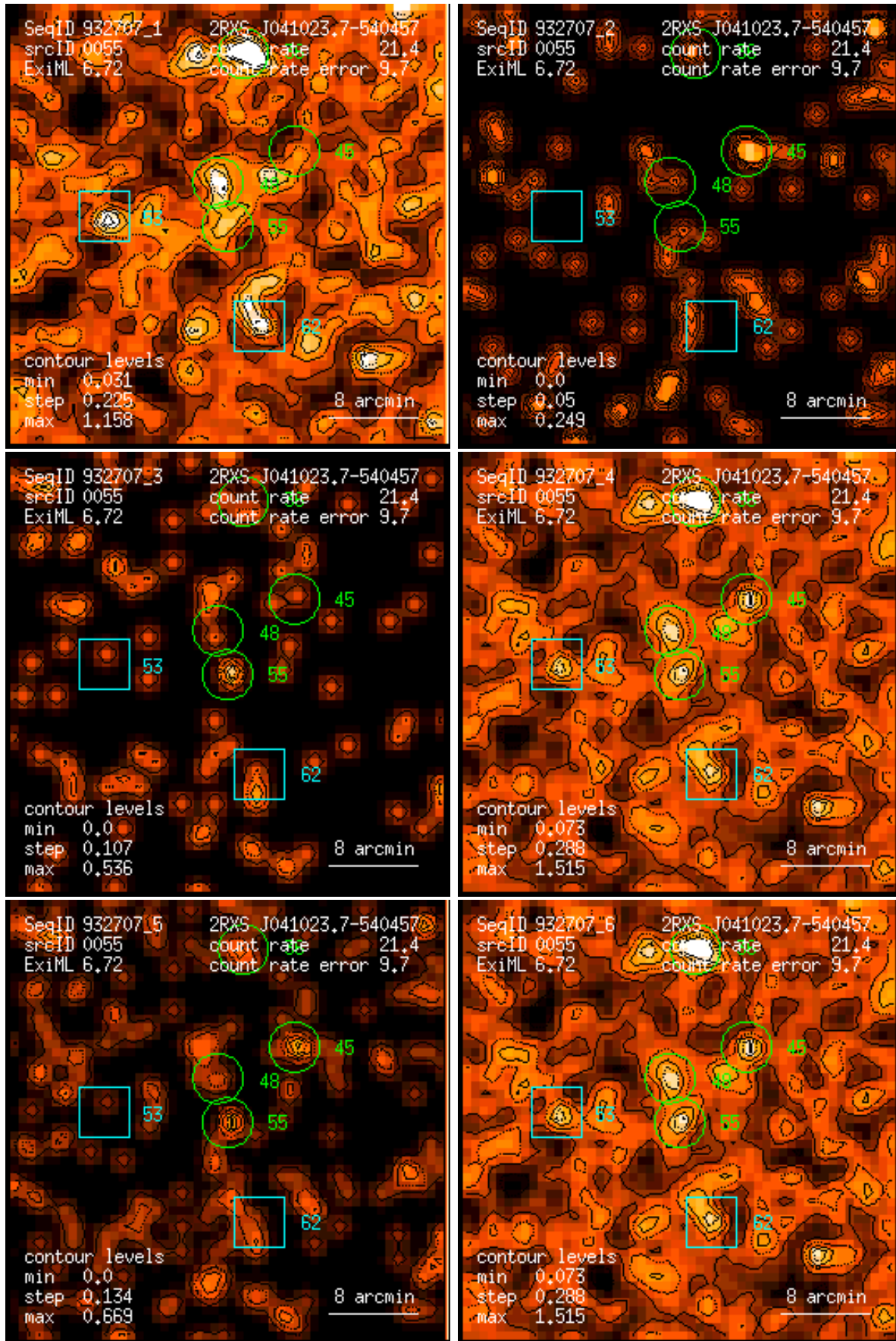
Figure 55: RASS 932707: detection 0055: band rate images, Gaussian filter: (1) PSPC channels 11 – 41, (2) 52 – 90, (3) 91 – 201, (4) 11 – 235, (5) 52 – 201, (6) 11 – 201. Broad band rates in counts/ks. Band rate contour levels in counts/ks/arcmin 2 .
