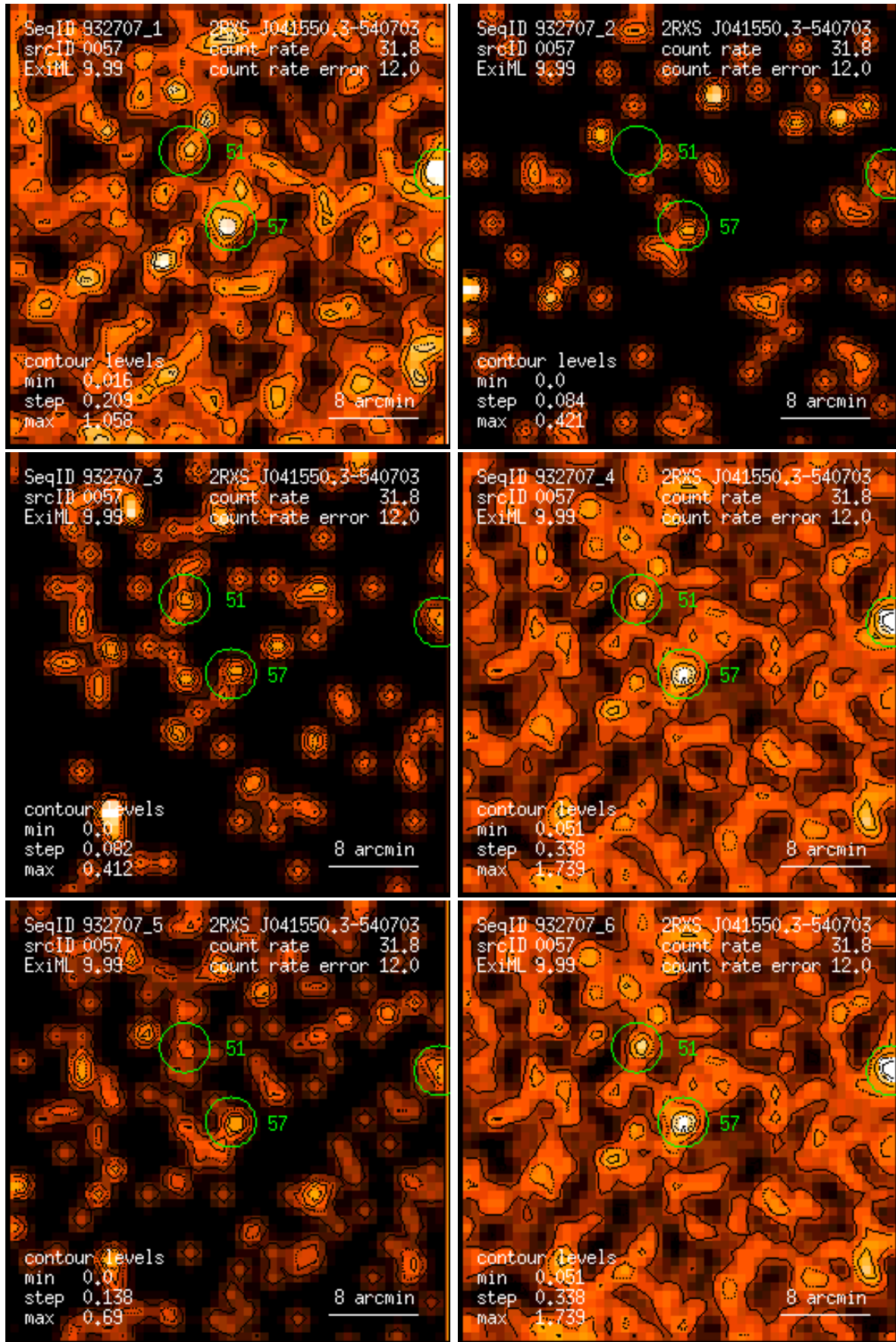
Figure 57: RASS 932707: detection 0057: band rate images, Gaussian filter: (1) PSPC channels 11 – 41, (2) 52 – 90, (3) 91 – 201, (4) 11 – 235, (5) 52 – 201, (6) 11 – 201. Broad band rates in counts/ks. Band rate contour levels in counts/ks/arcmin 2 .
