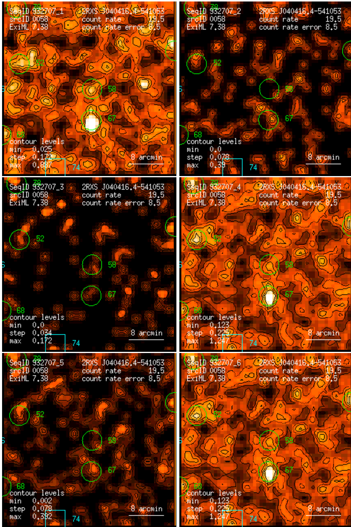
Figure 58: RASS 932707: detection 0058: band rate images, Gaussian filter: (1) PSPC channels 11 – 41, (2) 52 – 90, (3) 91 – 201, (4) 11 – 235, (5) 52 – 201, (6) 11 – 201. Broad band rates in counts/ks. Band rate contour levels in counts/ks/arcmin 2 .
