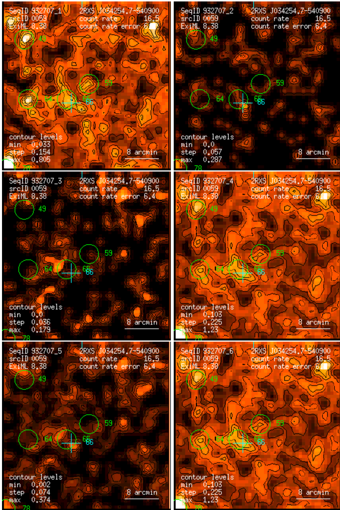
Figure 59: RASS 932707: detection 0059: band rate images, Gaussian filter: (1) PSPC channels 11 – 41, (2) 52 – 90, (3) 91 – 201, (4) 11 – 235, (5) 52 – 201, (6) 11 – 201. Broad band rates in counts/ks. Band rate contour levels in counts/ks/arcmin 2 .
