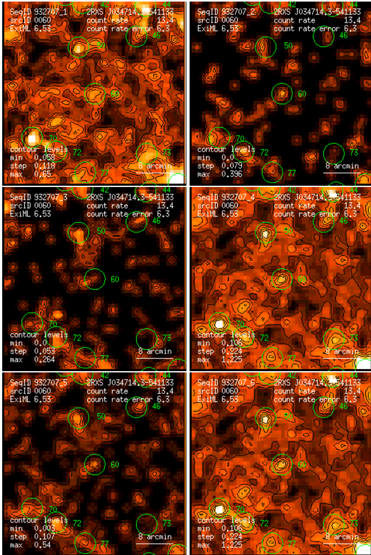
Figure 60: RASS 932707: detection 0060: band rate images, Gaussian filter: (1) PSPC channels 11 – 41, (2) 52 – 90, (3) 91 – 201, (4) 11 – 235, (5) 52 – 201, (6) 11 – 201. Broad band rates in counts/ks. Band rate contour levels in counts/ks/arcmin 2 .
