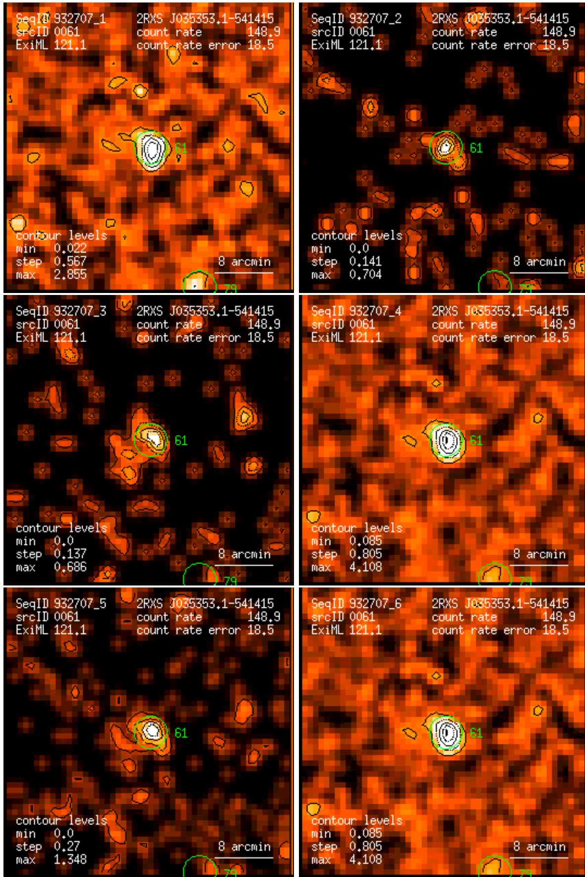
Figure 61: RASS 932707: detection 0061: band rate images, Gaussian filter: (1) PSPC channels 11 – 41, (2) 52 – 90, (3) 91 – 201, (4) 11 – 235, (5) 52 – 201, (6) 11 – 201. Broad band rates in counts/ks. Band rate contour levels in counts/ks/arcmin 2 .
