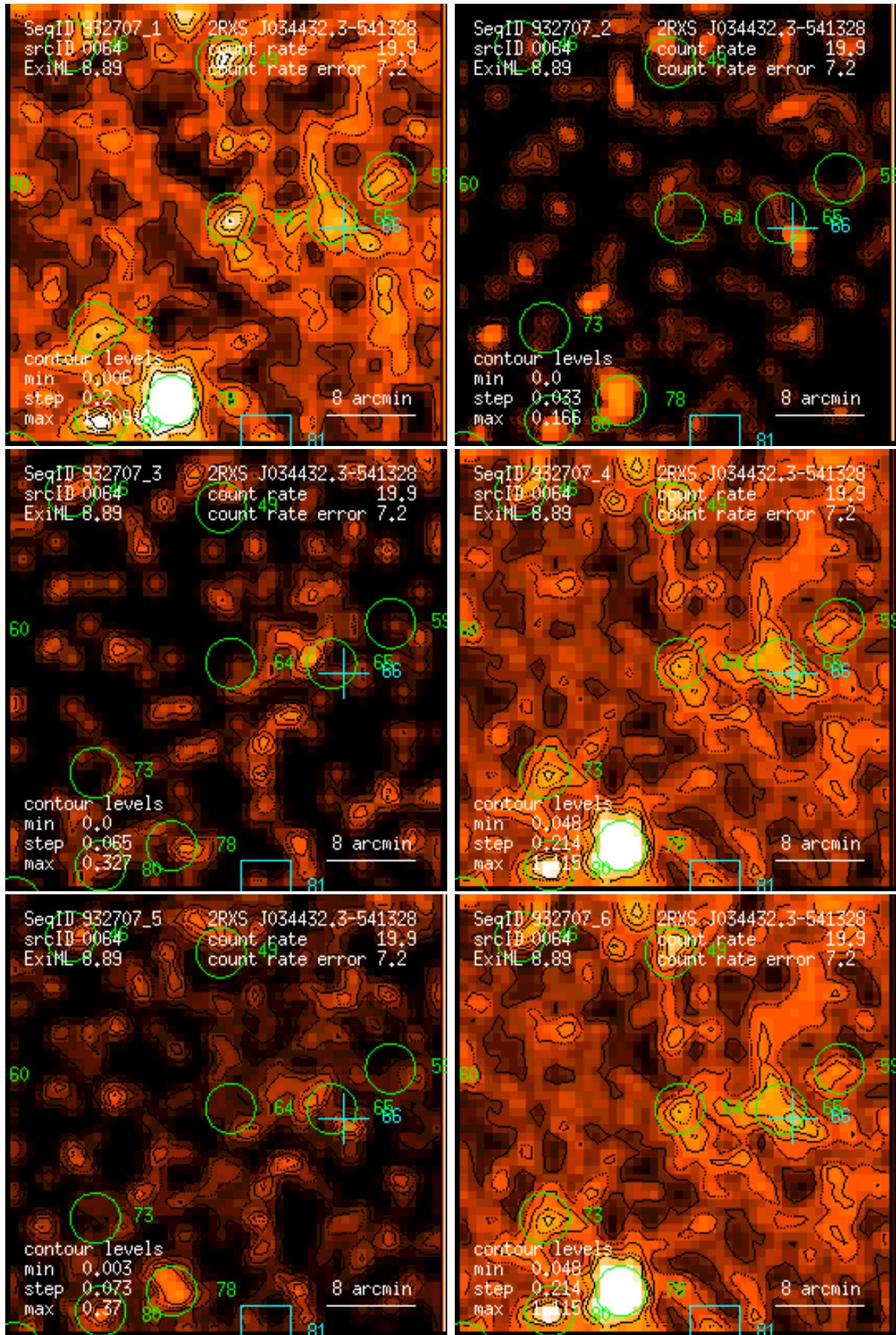
Figure 64: RASS 932707: detection 0064: band rate images, Gaussian filter: (1) PSPC channels 11 – 41, (2) 52 – 90, (3) 91 – 201, (4) 11 – 235, (5) 52 – 201, (6) 11 – 201. Broad band rates in counts/ks. Band rate contour levels in counts/ks/arcmin 2 .
