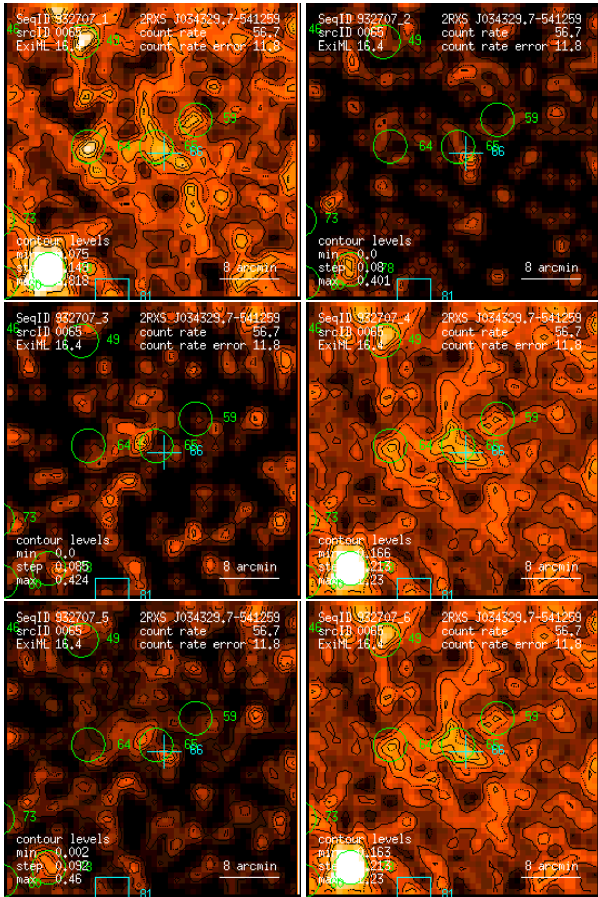
Figure 65: RASS 932707: detection 0065: band rate images, Gaussian filter: (1) PSPC channels 11 – 41, (2) 52 – 90, (3) 91 – 201, (4) 11 – 235, (5) 52 – 201, (6) 11 – 201. Broad band rates in counts/ks. Band rate contour levels in counts/ks/arcmin 2 .
