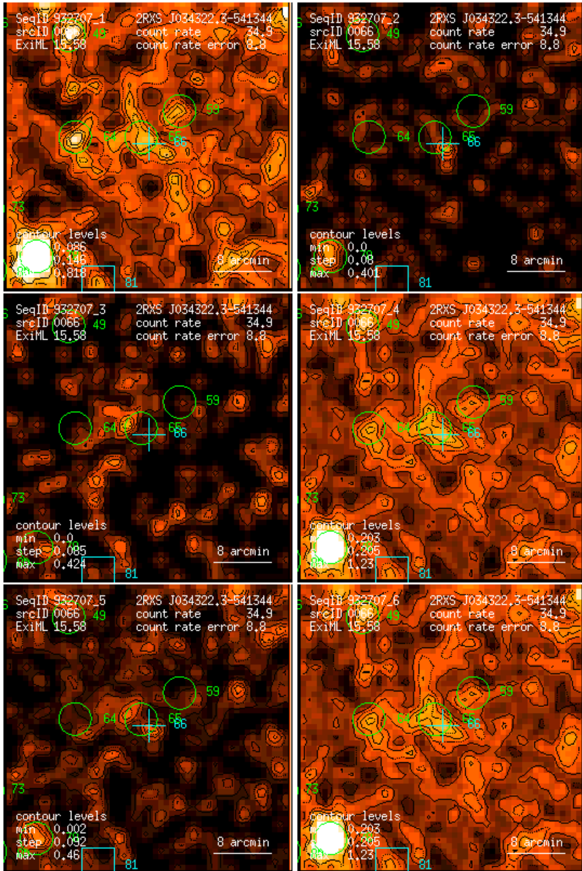
Figure 66: RASS 932707: detection 0066: band rate images, Gaussian filter: (1) PSPC channels 11 – 41, (2) 52 – 90, (3) 91 – 201, (4) 11 – 235, (5) 52 – 201, (6) 11 – 201. Broad band rates in counts/ks. Band rate contour levels in counts/ks/arcmin 2 .
