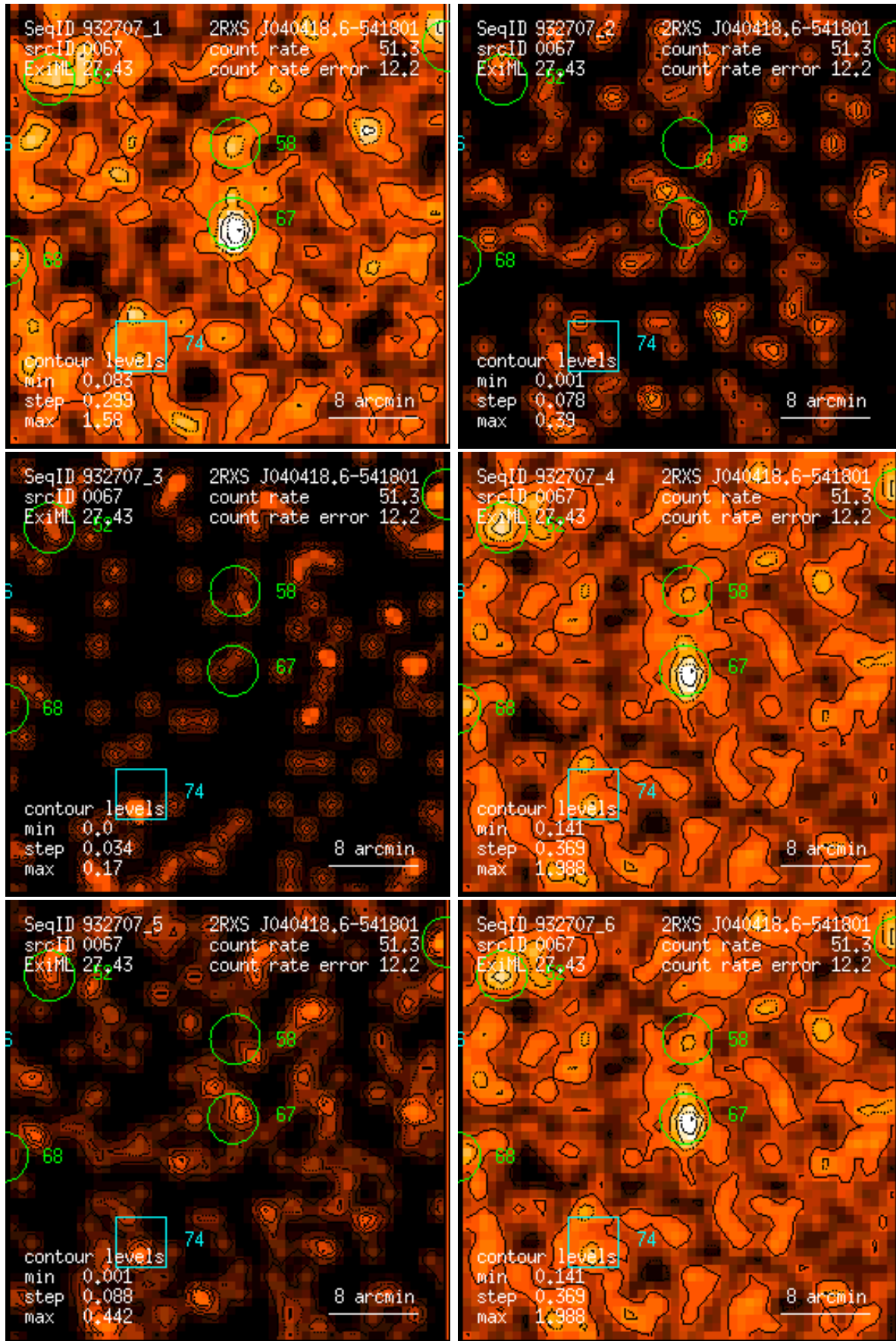
Figure 67: RASS 932707: detection 0067: band rate images, Gaussian filter: (1) PSPC channels 11 – 41, (2) 52 – 90, (3) 91 – 201, (4) 11 – 235, (5) 52 – 201, (6) 11 – 201. Broad band rates in counts/ks. Band rate contour levels in counts/ks/arcmin 2 .
