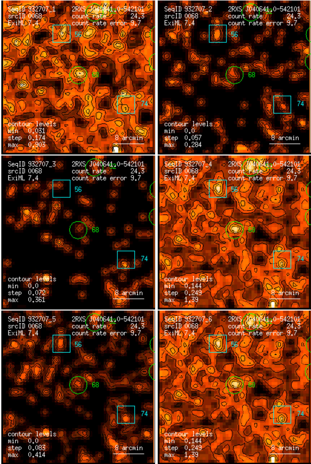
Figure 68: RASS 932707: detection 0068: band rate images, Gaussian filter: (1) PSPC channels 11 – 41, (2) 52 – 90, (3) 91 – 201, (4) 11 – 235, (5) 52 – 201, (6) 11 – 201. Broad band rates in counts/ks. Band rate contour levels in counts/ks/arcmin 2 .
