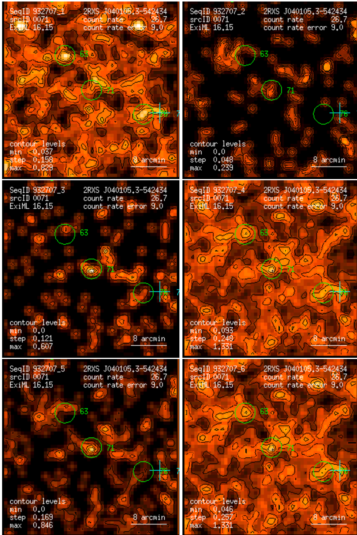
Figure 71: RASS 932707: detection 0071: band rate images, Gaussian filter: (1) PSPC channels 11 – 41, (2) 52 – 90, (3) 91 – 201, (4) 11 – 235, (5) 52 – 201, (6) 11 – 201. Broad band rates in counts/ks. Band rate contour levels in counts/ks/arcmin 2 .
