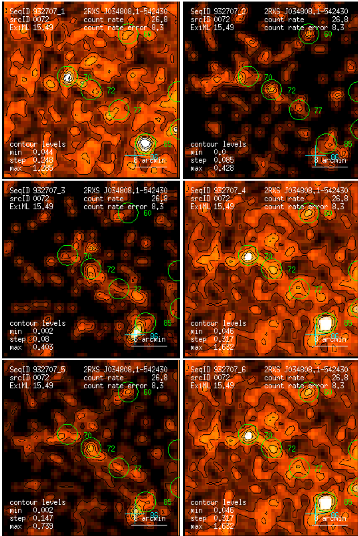
Figure 72: RASS 932707: detection 0072: band rate images, Gaussian filter: (1) PSPC channels 11 – 41, (2) 52 – 90, (3) 91 – 201, (4) 11 – 235, (5) 52 – 201, (6) 11 – 201. Broad band rates in counts/ks. Band rate contour levels in counts/ks/arcmin 2 .
