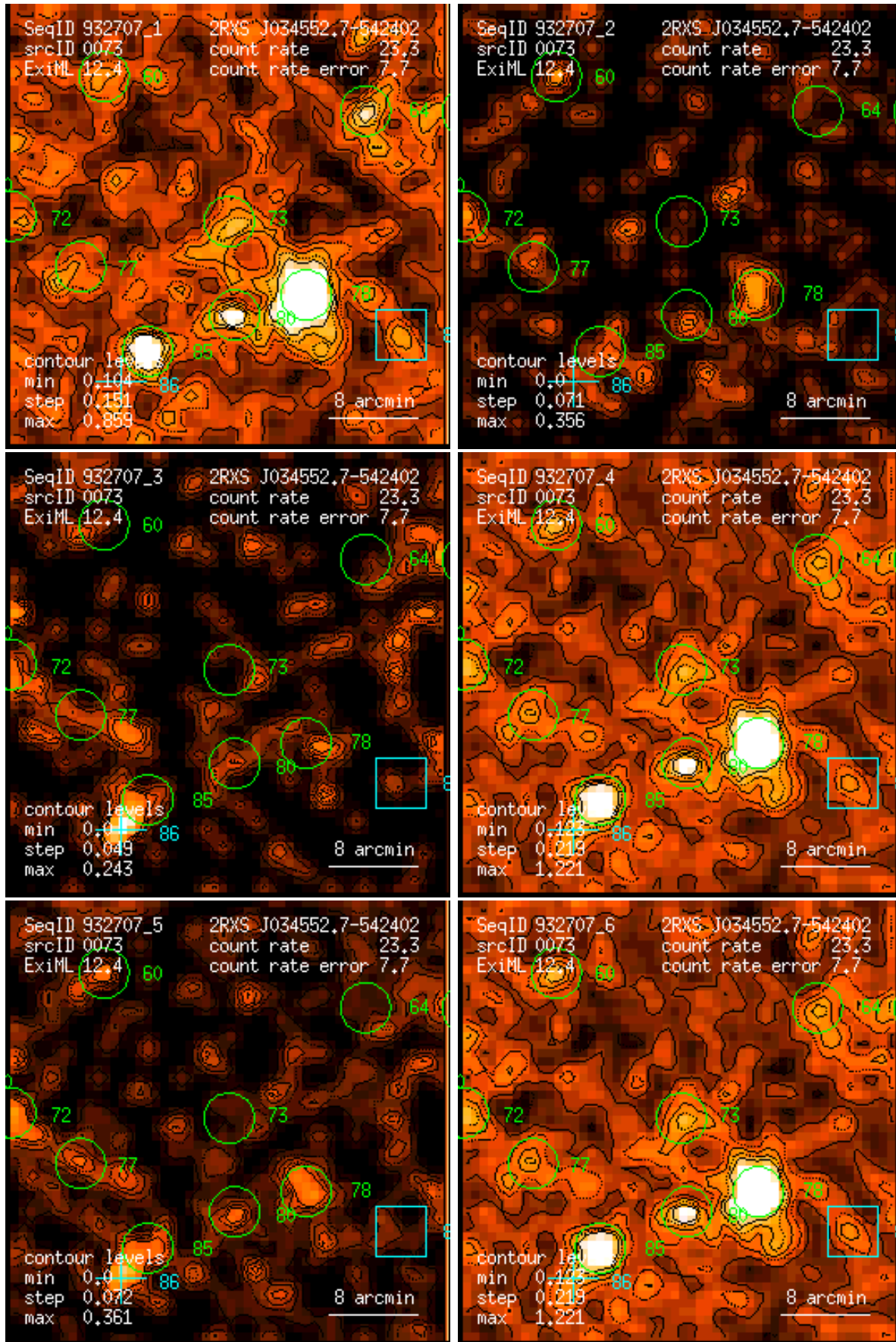
Figure 73: RASS 932707: detection 0073: band rate images, Gaussian filter: (1) PSPC channels 11 – 41, (2) 52 – 90, (3) 91 – 201, (4) 11 – 235, (5) 52 – 201, (6) 11 – 201. Broad band rates in counts/ks. Band rate contour levels in counts/ks/arcmin 2 .
