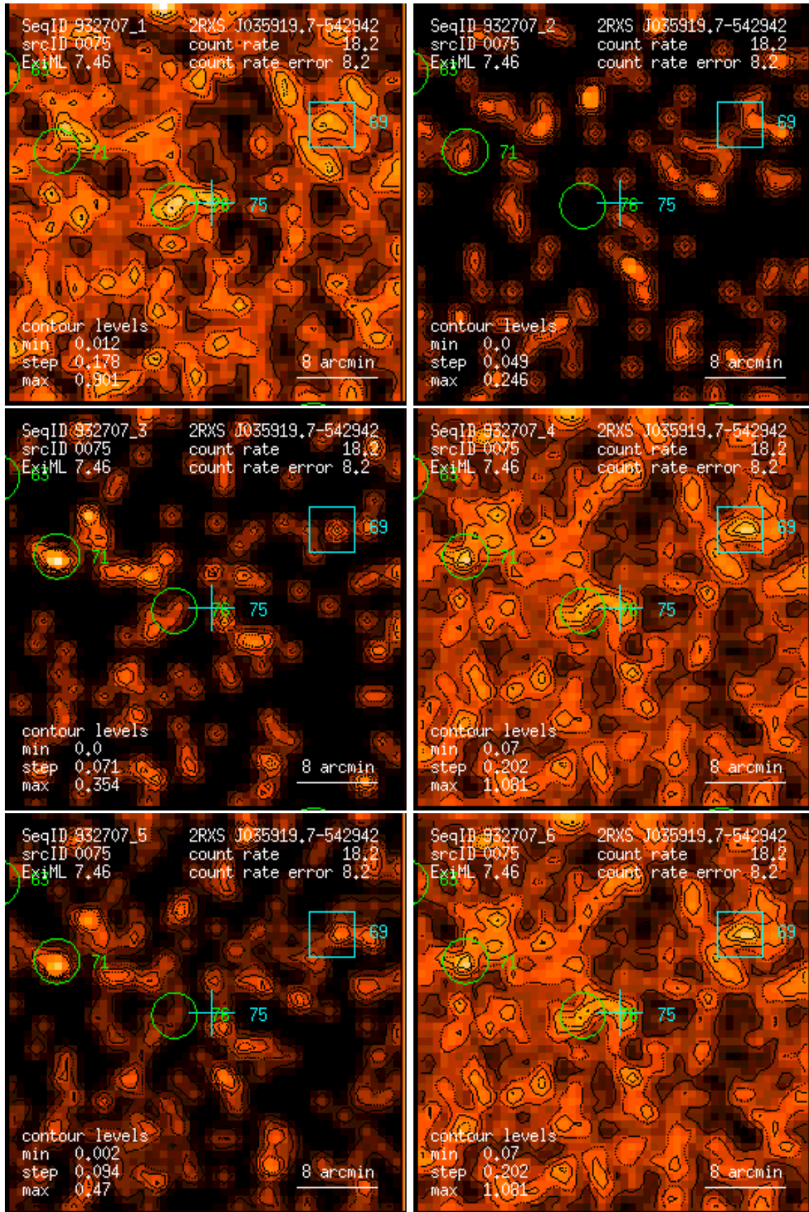
Figure 75: RASS 932707: detection 0075: band rate images, Gaussian filter: (1) PSPC channels 11 – 41, (2) 52 – 90, (3) 91 – 201, (4) 11 – 235, (5) 52 – 201, (6) 11 – 201. Broad band rates in counts/ks. Band rate contour levels in counts/ks/arcmin 2 .
