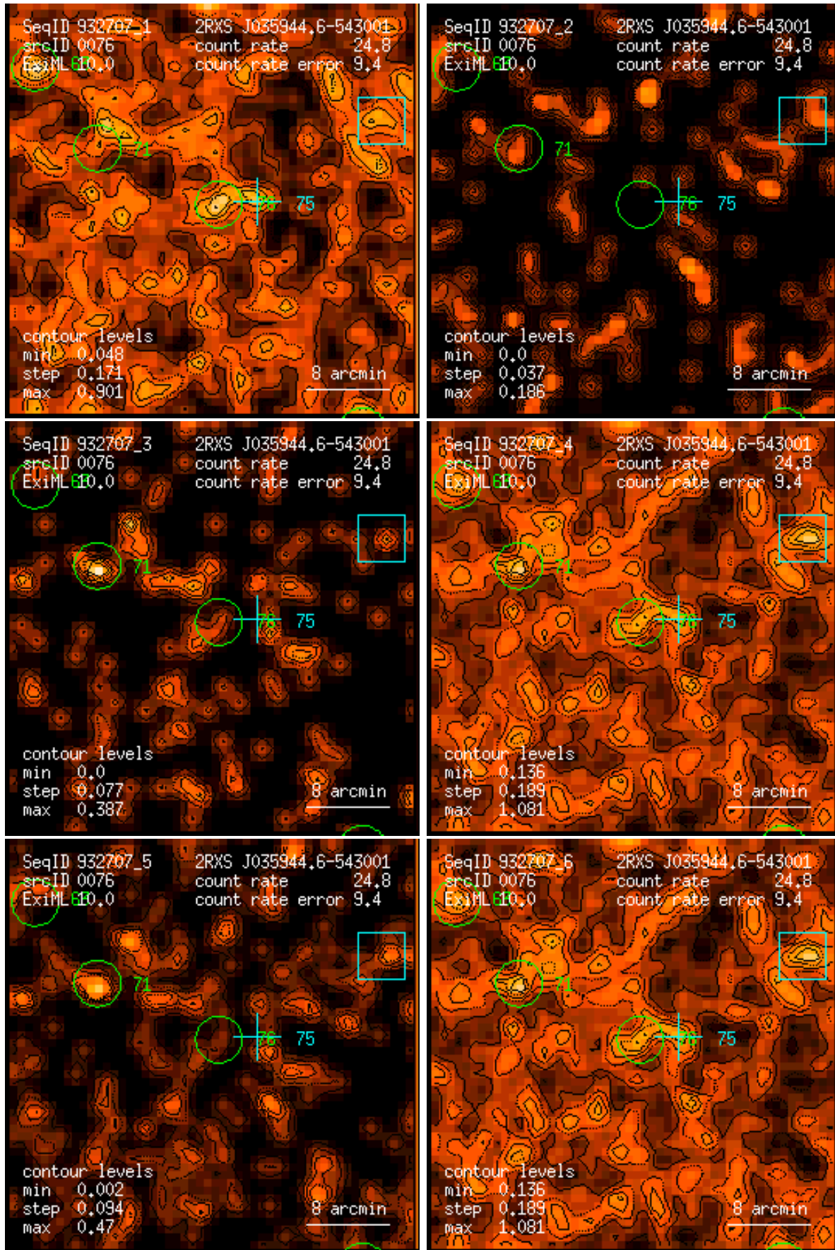
Figure 76: RASS 932707: detection 0076: band rate images, Gaussian filter: (1) PSPC channels 11 – 41, (2) 52 – 90, (3) 91 – 201, (4) 11 – 235, (5) 52 – 201, (6) 11 – 201. Broad band rates in counts/ks. Band rate contour levels in counts/ks/arcmin 2 .
