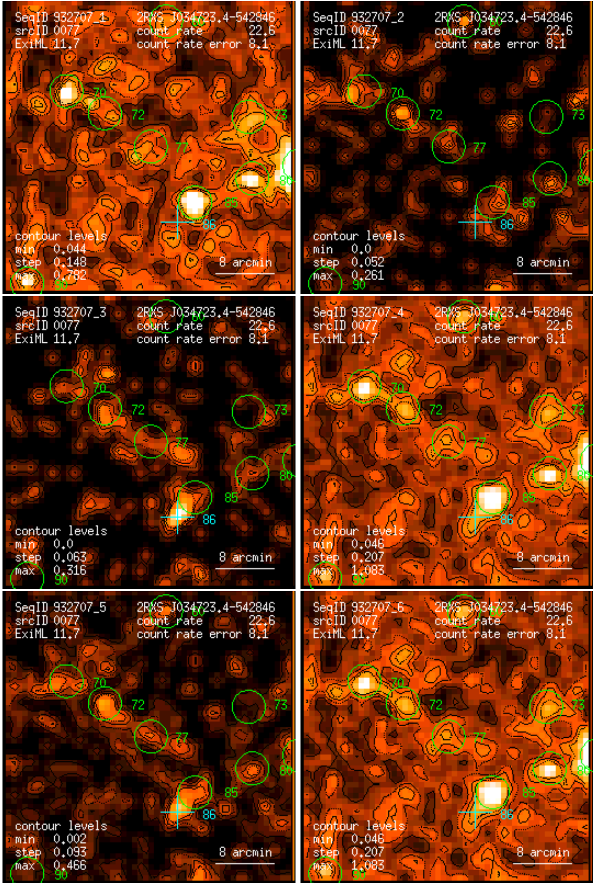
Figure 77: RASS 932707: detection 0077: band rate images, Gaussian filter: (1) PSPC channels 11 – 41, (2) 52 – 90, (3) 91 – 201, (4) 11 – 235, (5) 52 – 201, (6) 11 – 201. Broad band rates in counts/ks. Band rate contour levels in counts/ks/arcmin 2 .
