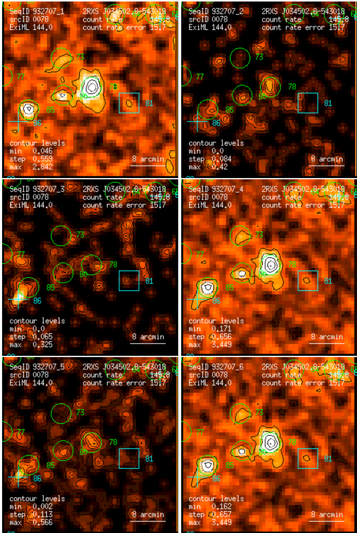
Figure 78: RASS 932707: detection 0078: band rate images, Gaussian filter: (1) PSPC channels 11 – 41, (2) 52 – 90, (3) 91 – 201, (4) 11 – 235, (5) 52 – 201, (6) 11 – 201. Broad band rates in counts/ks. Band rate contour levels in counts/ks/arcmin 2 .
