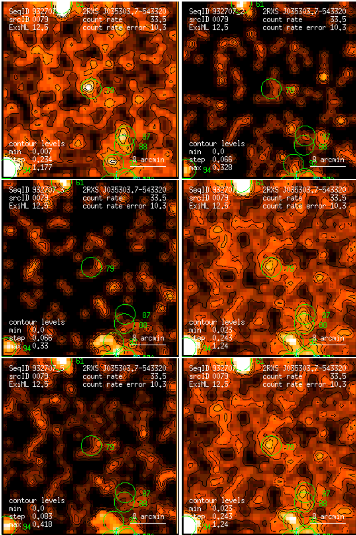
Figure 79: RASS 932707: detection 0079: band rate images, Gaussian filter: (1) PSPC channels 11 – 41, (2) 52 – 90, (3) 91 – 201, (4) 11 – 235, (5) 52 – 201, (6) 11 – 201. Broad band rates in counts/ks. Band rate contour levels in counts/ks/arcmin 2 .
