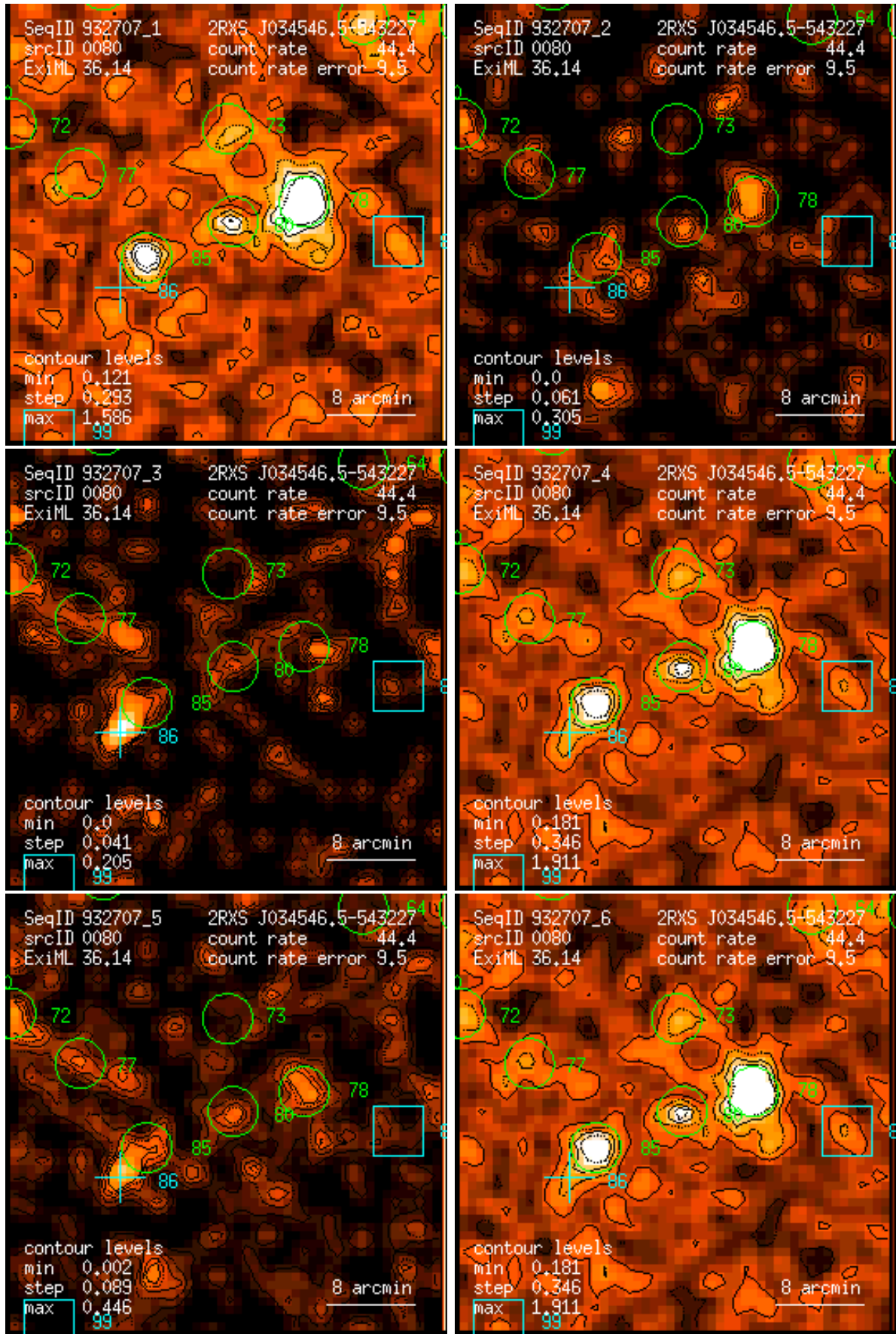
Figure 80: RASS 932707: detection 0080: band rate images, Gaussian filter: (1) PSPC channels 11 – 41, (2) 52 – 90, (3) 91 – 201, (4) 11 – 235, (5) 52 – 201, (6) 11 – 201. Broad band rates in counts/ks. Band rate contour levels in counts/ks/arcmin 2 .
