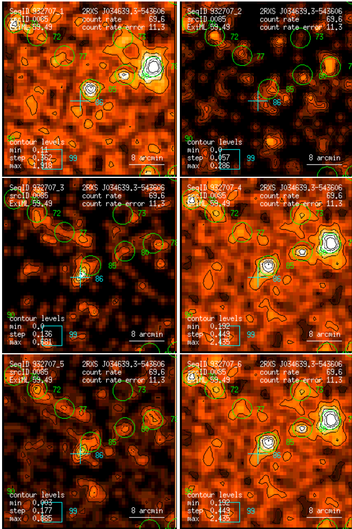
Figure 85: RASS 932707: detection 0085: band rate images, Gaussian filter: (1) PSPC channels 11 – 41, (2) 52 – 90, (3) 91 – 201, (4) 11 – 235, (5) 52 – 201, (6) 11 – 201. Broad band rates in counts/ks. Band rate contour levels in counts/ks/arcmin 2 .
