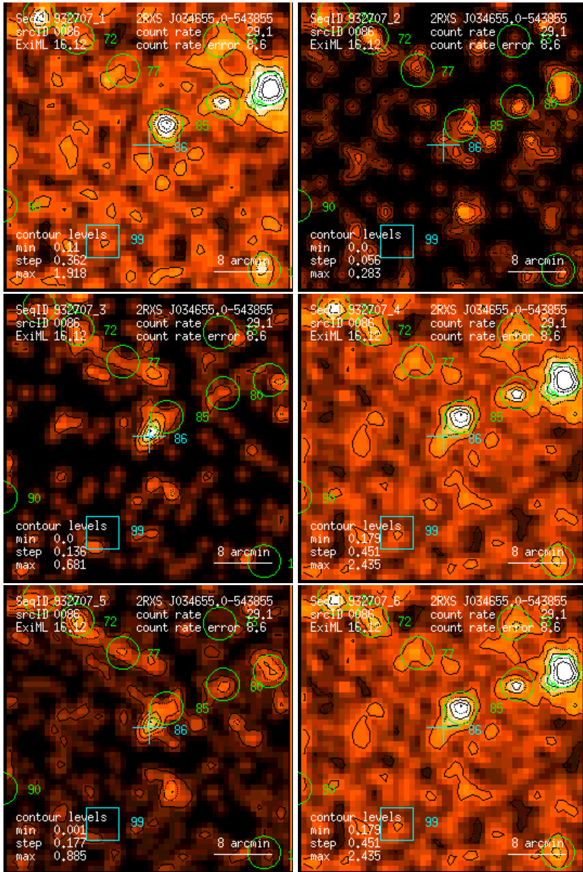
Figure 86: RASS 932707: detection 0086: band rate images, Gaussian filter: (1) PSPC channels 11 – 41, (2) 52 – 90, (3) 91 – 201, (4) 11 – 235, (5) 52 – 201, (6) 11 – 201. Broad band rates in counts/ks. Band rate contour levels in counts/ks/arcmin 2 .
