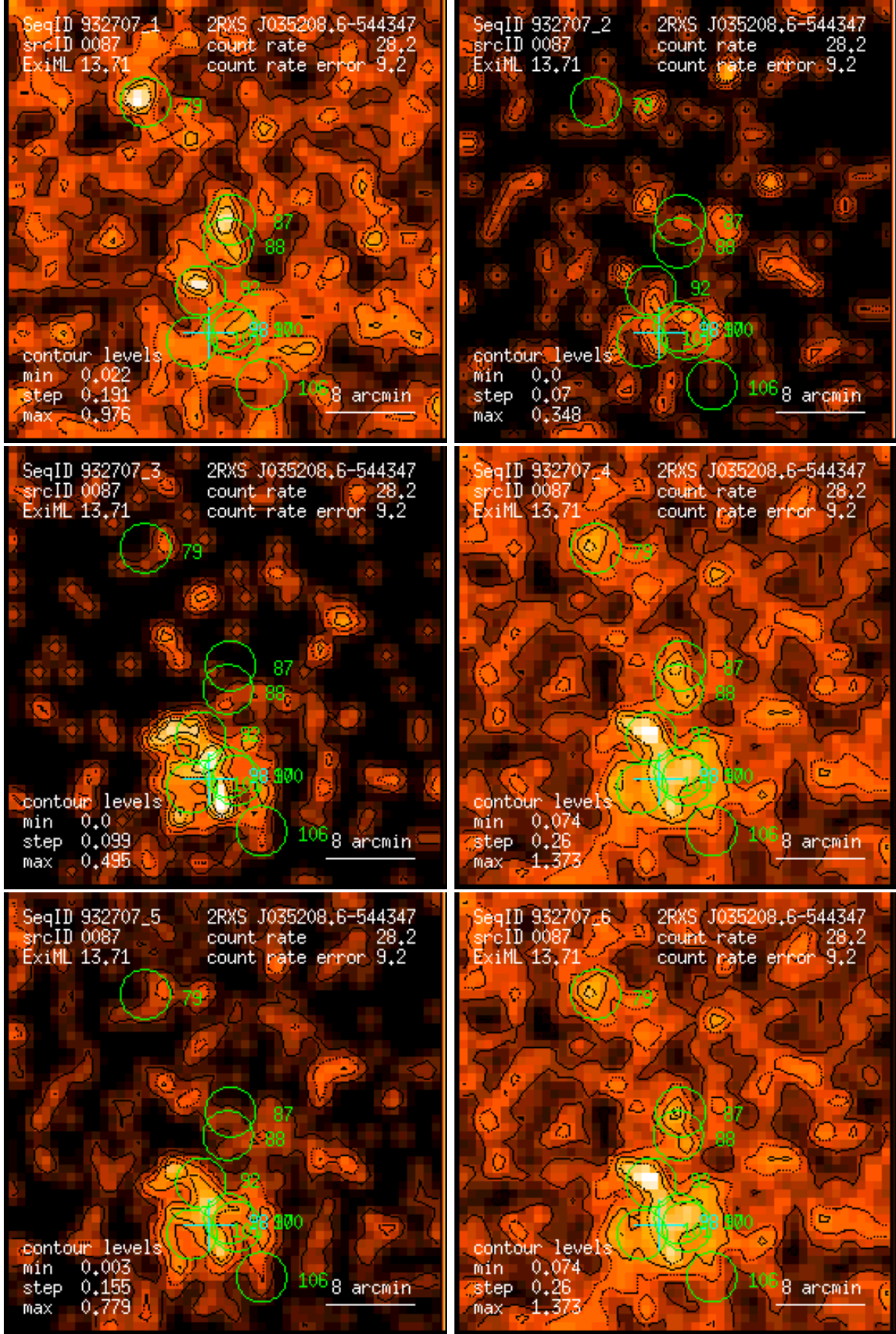
Figure 87: RASS 932707: detection 0087: band rate images, Gaussian filter: (1) PSPC channels 11 – 41, (2) 52 – 90, (3) 91 – 201, (4) 11 – 235, (5) 52 – 201, (6) 11 – 201. Broad band rates in counts/ks. Band rate contour levels in counts/ks/arcmin 2 .
