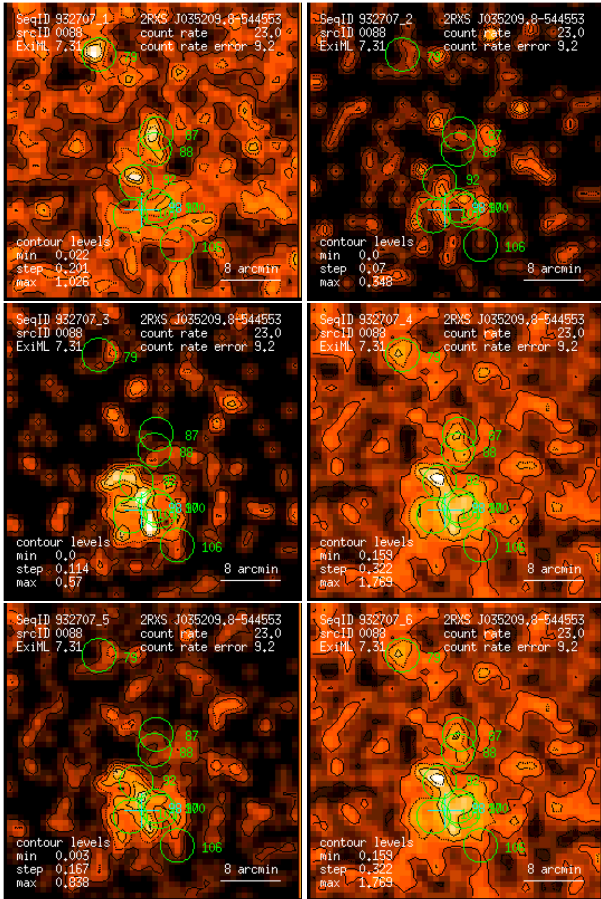
Figure 88: RASS 932707: detection 0088: band rate images, Gaussian filter: (1) PSPC channels 11 – 41, (2) 52 – 90, (3) 91 – 201, (4) 11 – 235, (5) 52 – 201, (6) 11 – 201. Broad band rates in counts/ks. Band rate contour levels in counts/ks/arcmin 2 .
