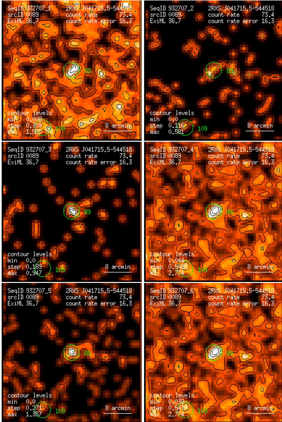
Figure 89: RASS 932707: detection 0089: band rate images, Gaussian filter: (1) PSPC channels 11 – 41, (2) 52 – 90, (3) 91 – 201, (4) 11 – 235, (5) 52 – 201, (6) 11 – 201. Broad band rates in counts/ks. Band rate contour levels in counts/ks/arcmin 2 .
