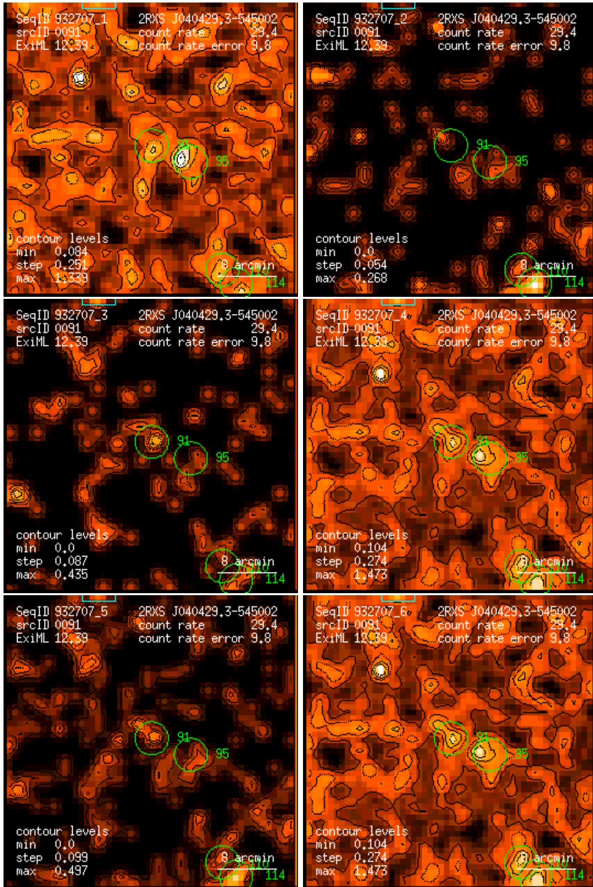
Figure 91: RASS 932707: detection 0091: band rate images, Gaussian filter: (1) PSPPC channels 11 – 41, (2) 52 – 90, (3) 91 – 201, (4) 11 – 235, (5) 52 – 201, (6) 11 – 201. Broad band rates in counts/ks. Band rate contour levels in counts/ks/arcmin 2 .
