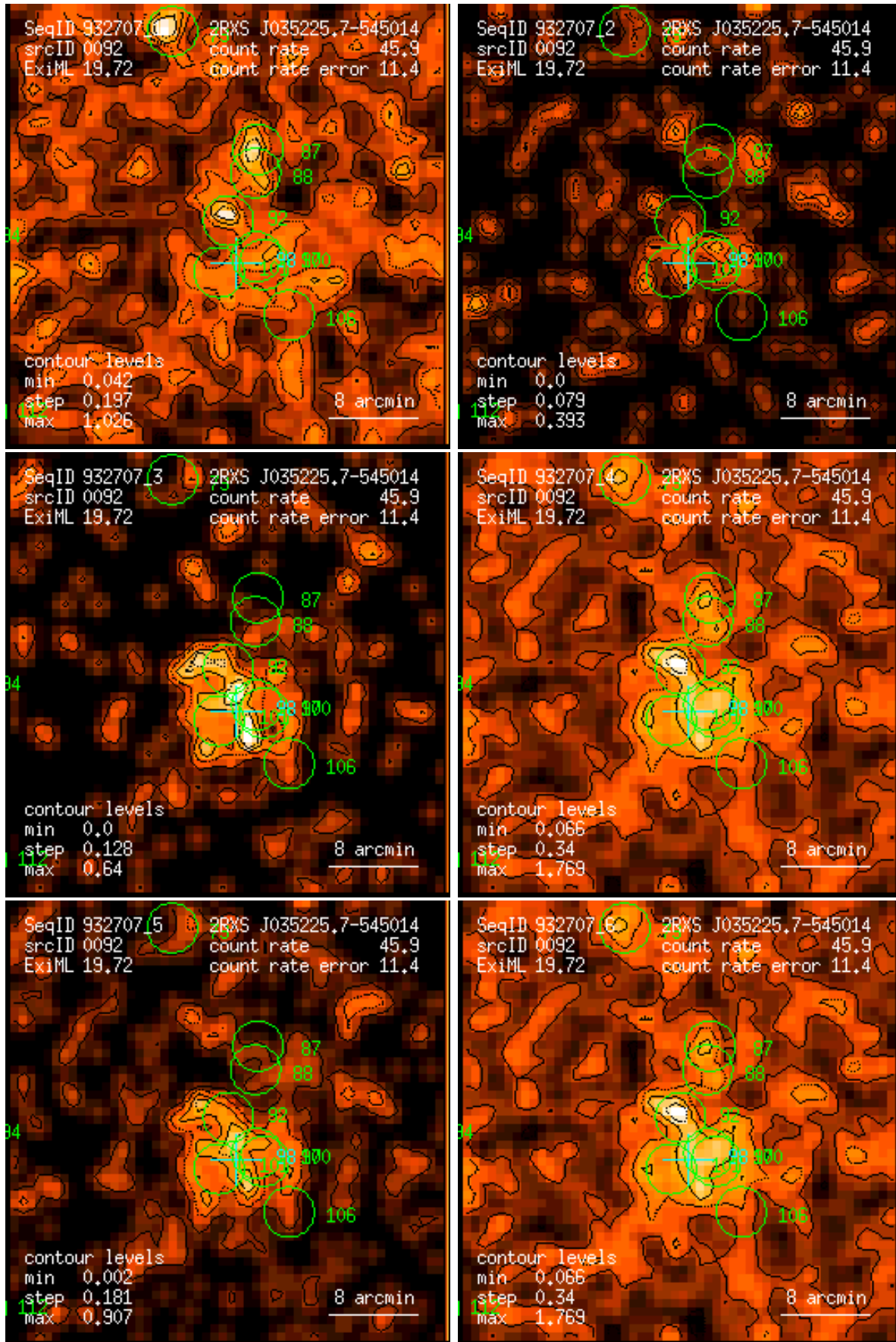
Figure 92: RASS 932707: detection 0092: band rate images, Gaussian filter: (1) PSPC channels 11 – 41, (2) 52 – 90, (3) 91 – 201, (4) 11 – 235, (5) 52 – 201, (6) 11 – 201. Broad band rates in counts/ks. Band rate contour levels in counts/ks/arcmin 2 .
