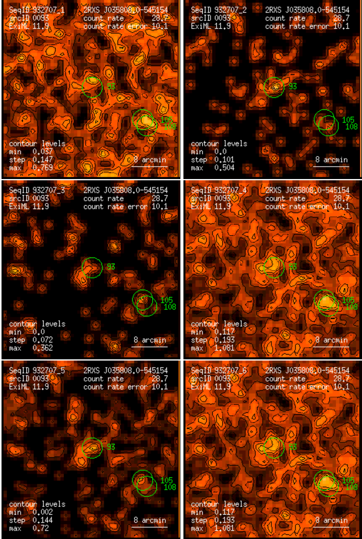
Figure 93: RASS 932707: detection 0093: band rate images, Gaussian filter: (1) PSPC channels 11 – 41, (2) 52 – 90, (3) 91 – 201, (4) 11 – 235, (5) 52 – 201, (6) 11 – 201. Broad band rates in counts/ks. Band rate contour levels in counts/ks/arcmin 2 .
