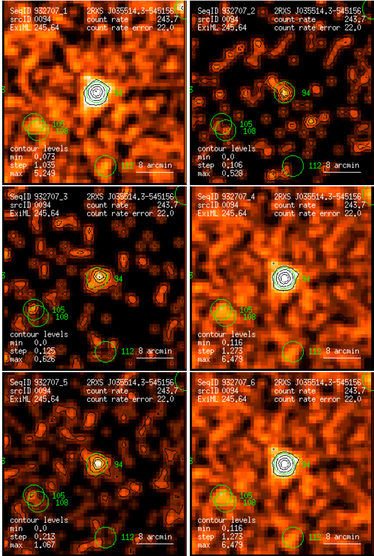
Figure 94: RASS 932707: detection 0094: band rate images, Gaussian filter: (1) PSPC channels 11 – 41, (2) 52 – 90, (3) 91 – 201, (4) 11 – 235, (5) 52 – 201, (6) 11 – 201. Broad band rates in counts/ks. Band rate contour levels in counts/ks/arcmin 2 .
