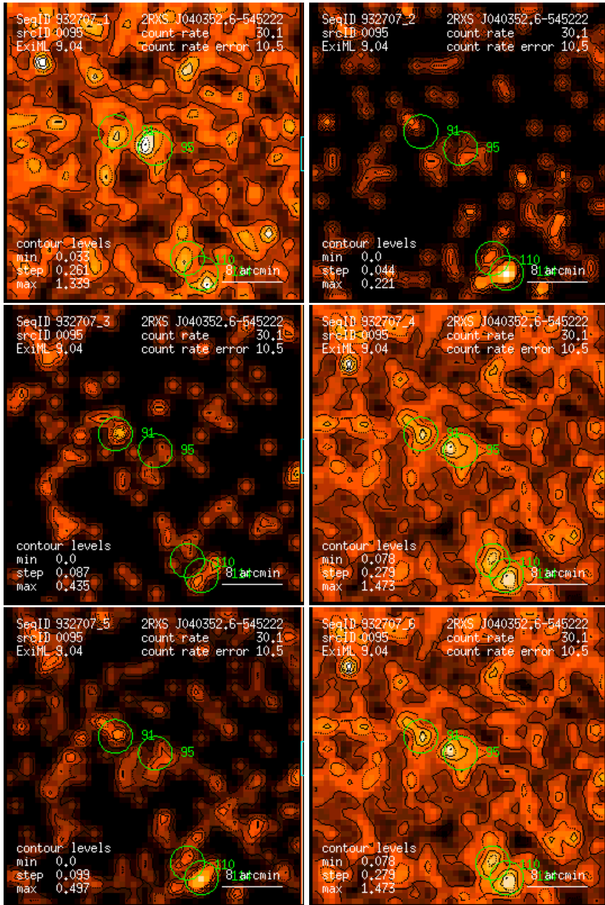
Figure 95: RASS 932707: detection 0095: band rate images, Gaussian filter: (1) PSPC channels 11 – 41, (2) 52 – 90, (3) 91 – 201, (4) 11 – 235, (5) 52 – 201, (6) 11 – 201. Broad band rates in counts/ks. Band rate contour levels in counts/ks/arcmin 2 .
