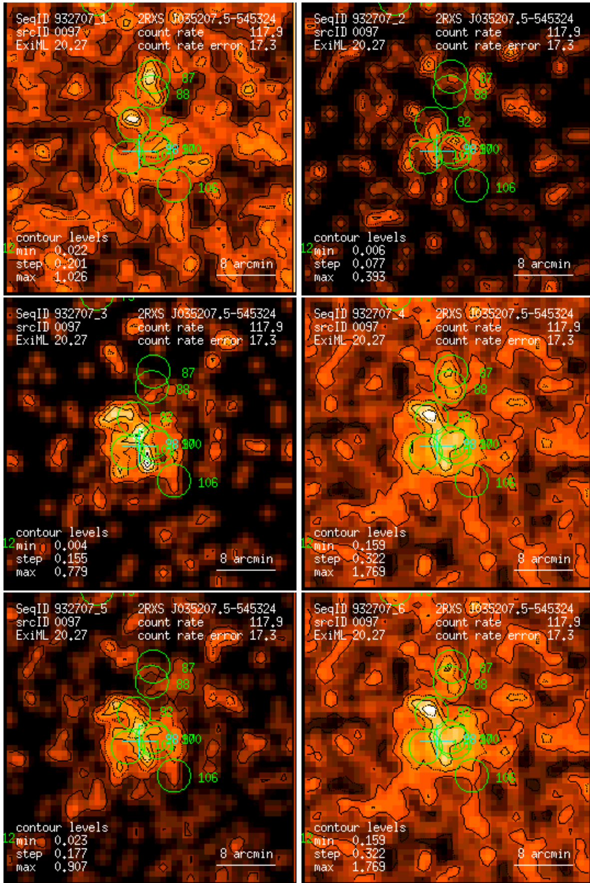
Figure 97: RASS 932707: detection 0097: band rate images, Gaussian filter: (1) PSPC channels 11 – 41, (2) 52 – 90, (3) 91 – 201, (4) 11 – 235, (5) 52 – 201, (6) 11 – 201. Broad band rates in counts/ks. Band rate contour levels in counts/ks/arcmin 2 .
