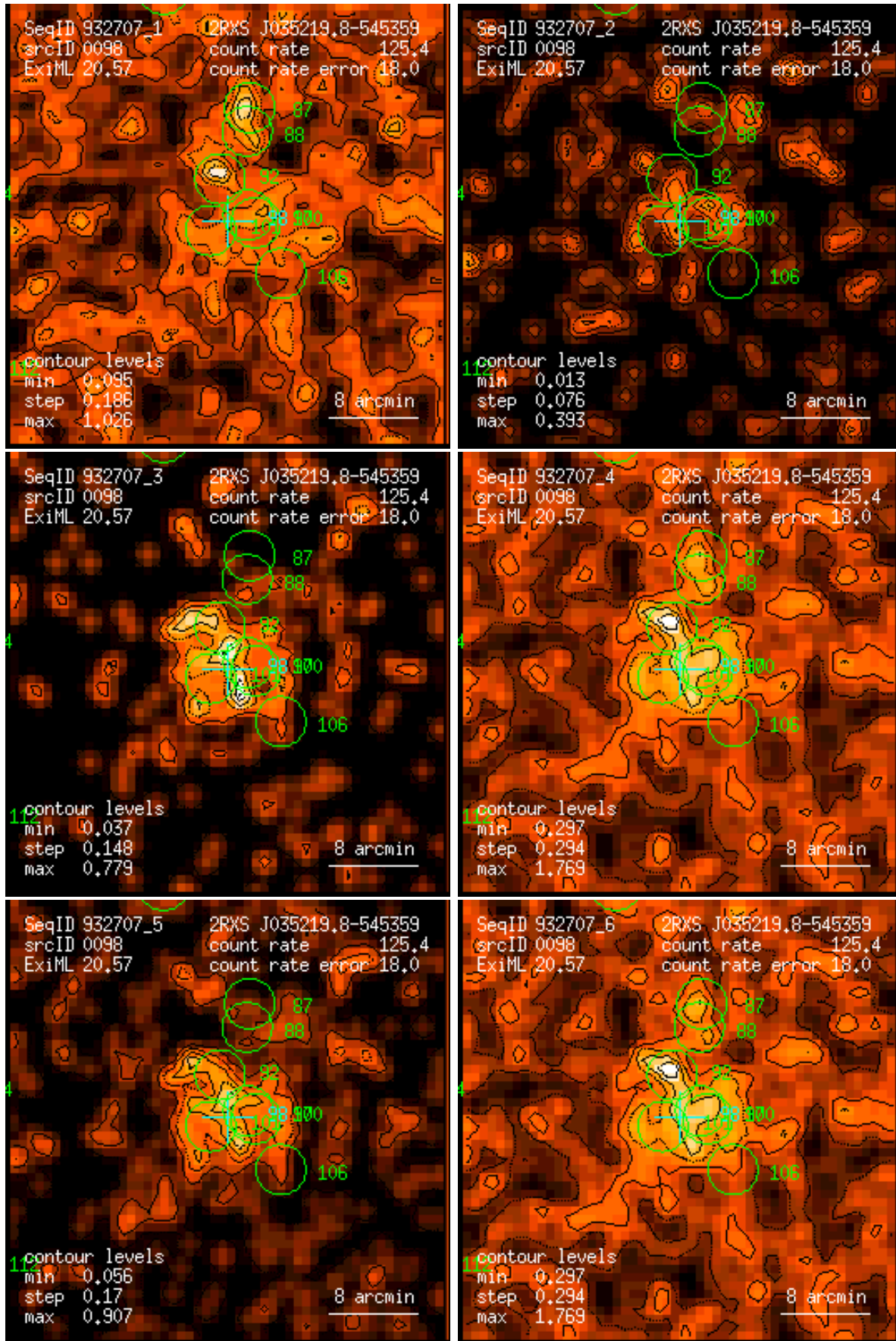
Figure 98: RASS 932707: detection 0098: band rate images, Gaussian filter: (1) PSPC channels 11 – 41, (2) 52 – 90, (3) 91 – 201, (4) 11 – 235, (5) 52 – 201, (6) 11 – 201. Broad band rates in counts/ks. Band rate contour levels in counts/ks/arcmin 2 .
