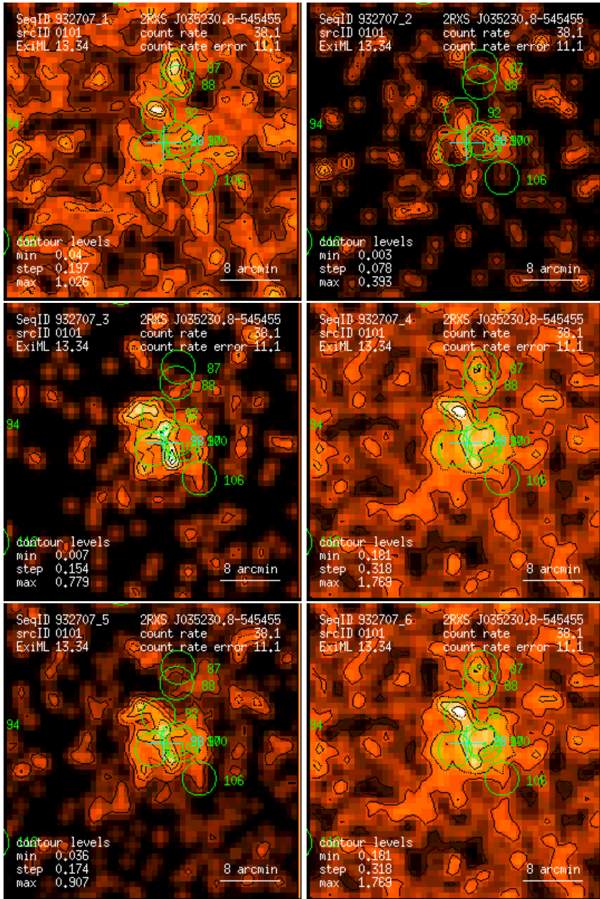
Figure 101: RASS 932707: detection 0101: band rate images, Gaussian filter: (1) PSPC channels 11 – 41, (2) 52 – 90, (3) 91 – 201, (4) 11 – 235, (5) 52 – 201, (6) 11 – 201. Broad band rates in counts/ks. Band rate contour levels in counts/ks/arcmin 2 .
