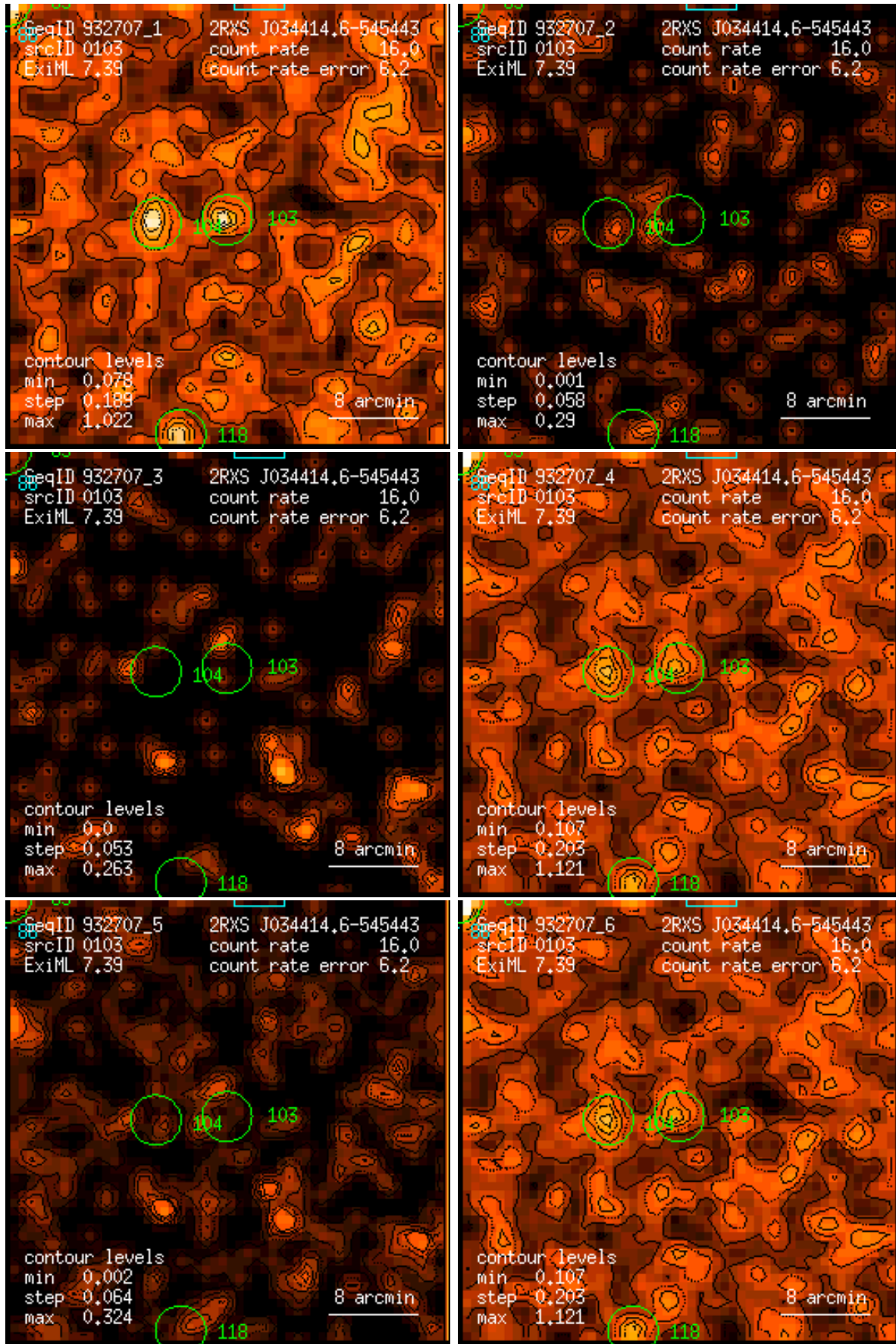
Figure 103: RASS 932707: detection 0103: band rate images, Gaussian filter: (1) PSPC channels 11 – 41, (2) 52 – 90, (3) 91 – 201, (4) 11 – 235, (5) 52 – 201, (6) 11 – 201. Broad band rates in counts/ks. Band rate contour levels in counts/ks/arcmin 2 .
