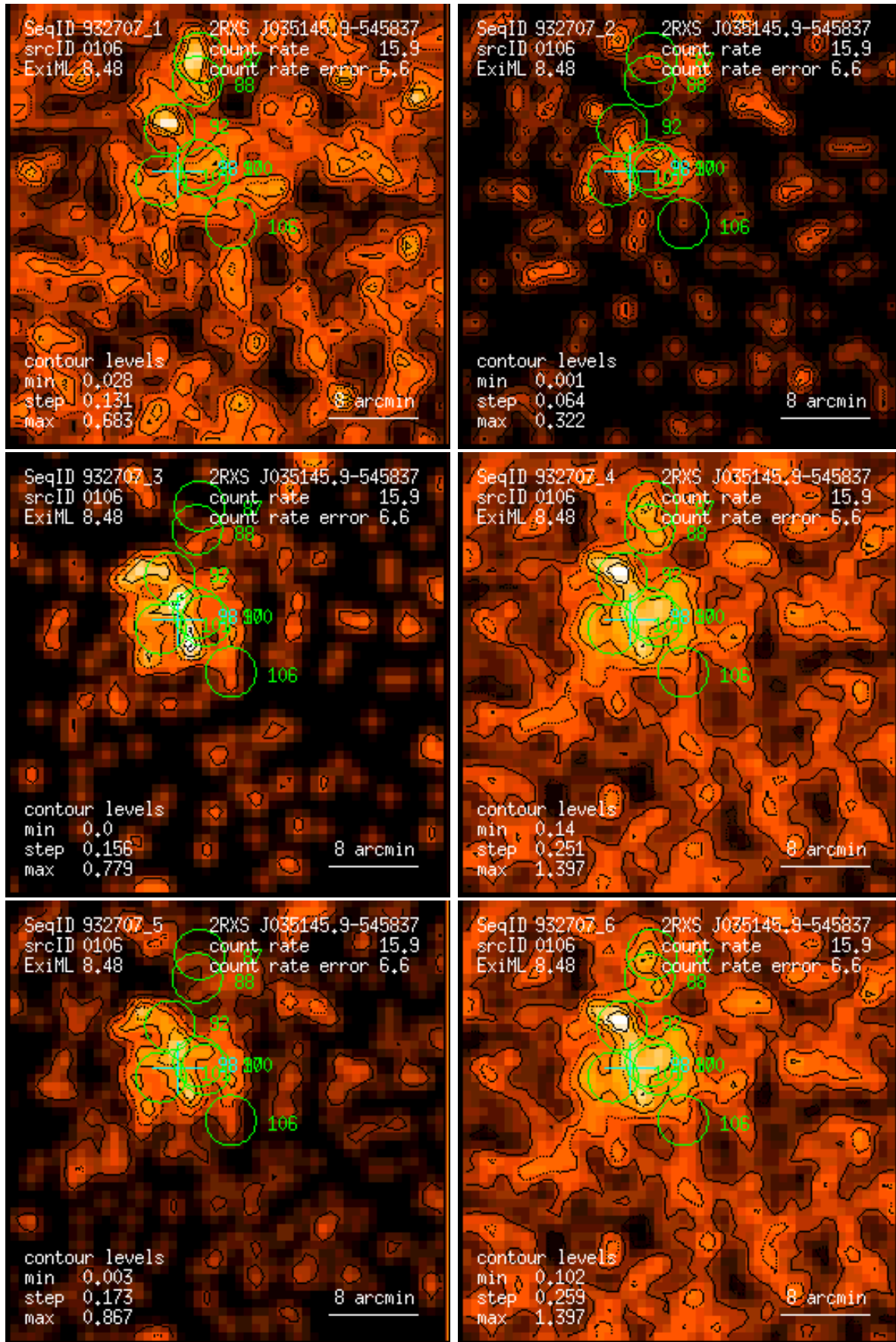
Figure 106: RASS 932707: detection 0106: band rate images, Gaussian filter: (1) PSPC channels 11 – 41, (2) 52 – 90, (3) 91 – 201, (4) 11 – 235, (5) 52 – 201, (6) 11 – 201. Broad band rates in counts/ks. Band rate contour levels in counts/ks/arcmin 2 .
