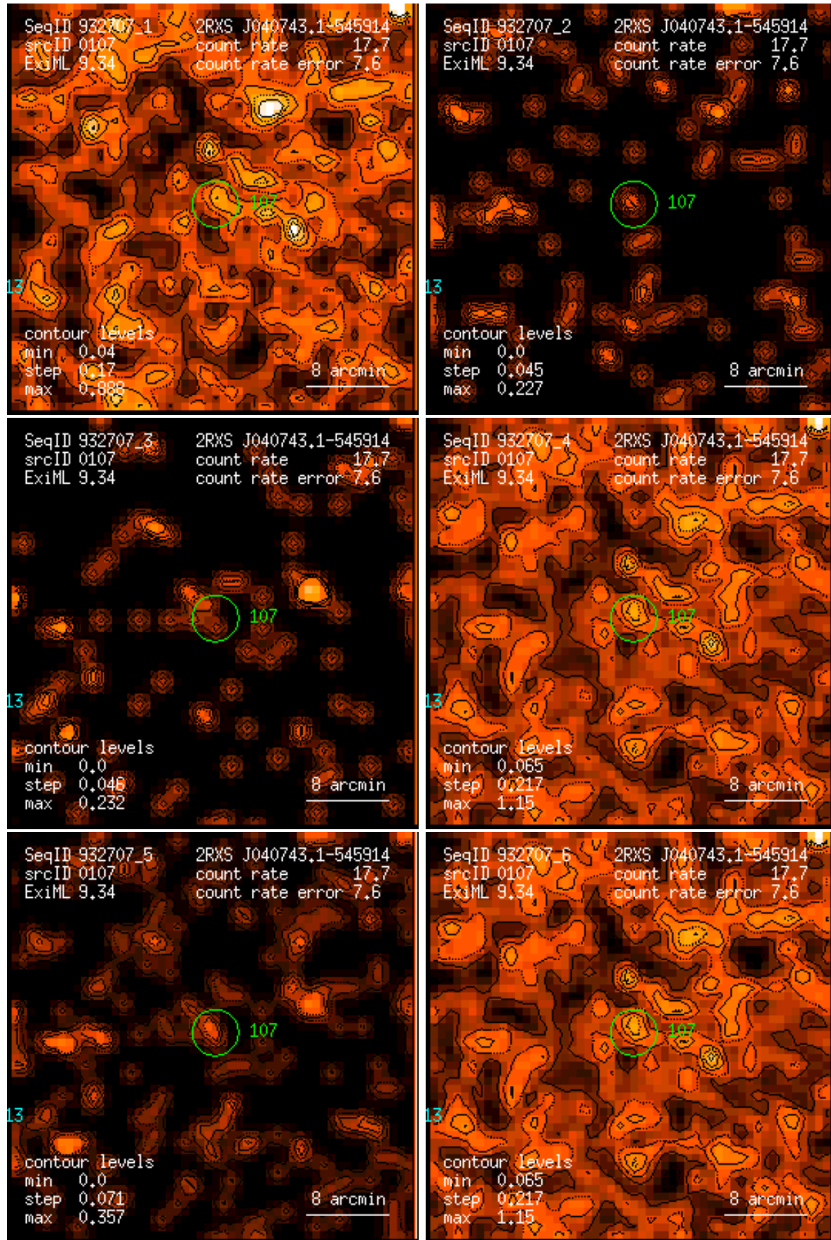
Figure 107: RASS 932707: detection 0107: band rate images, Gaussian filter: (1) PSPC channels 11 – 41, (2) 52 – 90, (3) 91 – 201, (4) 11 – 235, (5) 52 – 201, (6) 11 – 201. Broad band rates in counts/ks. Band rate contour levels in counts/ks/arcmin 2 .
