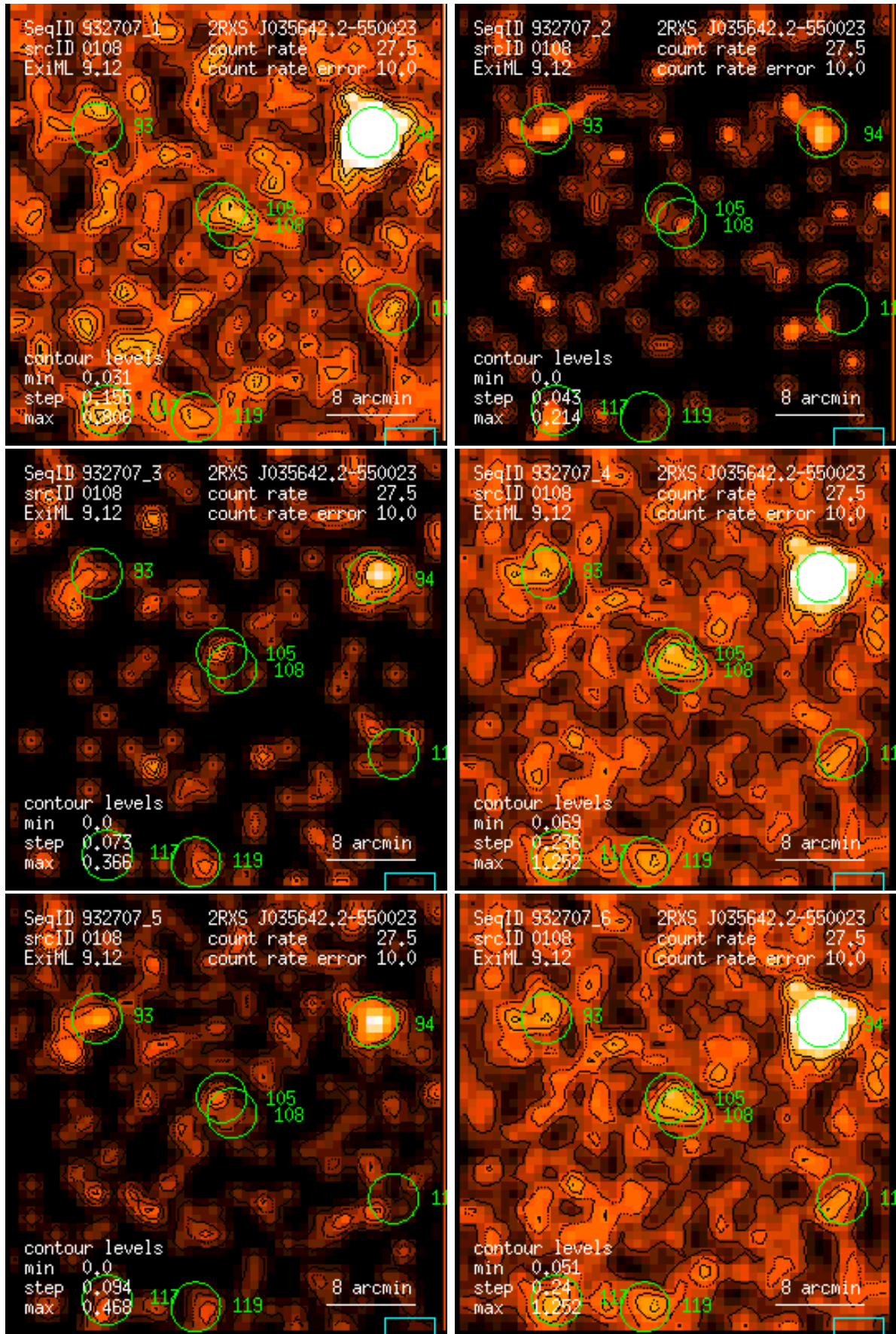
Figure 108: RASS 932707: detection 0108: band rate images, Gaussian filter: (1) PSPC channels 11 – 41, (2) 52 – 90, (3) 91 – 201, (4) 11 – 235, (5) 52 – 201, (6) 11 – 201. Broad band rates in counts/ks. Band rate contour levels in counts/ks/arcmin 2 .
