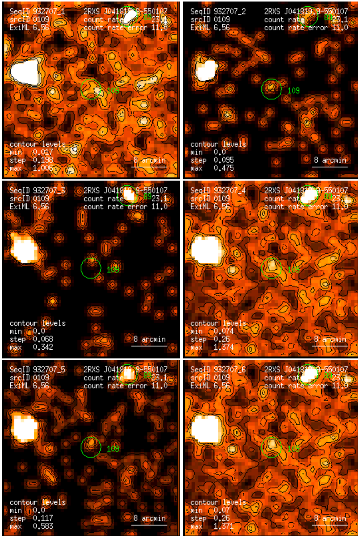
Figure 109: RASS 932707: detection 0109: band rate images, Gaussian filter: (1) PSPC channels 11 – 41, (2) 52 – 90, (3) 91 – 201, (4) 11 – 235, (5) 52 – 201, (6) 11 – 201. Broad band rates in counts/ks. Band rate contour levels in counts/ks/arcmin 2 .
