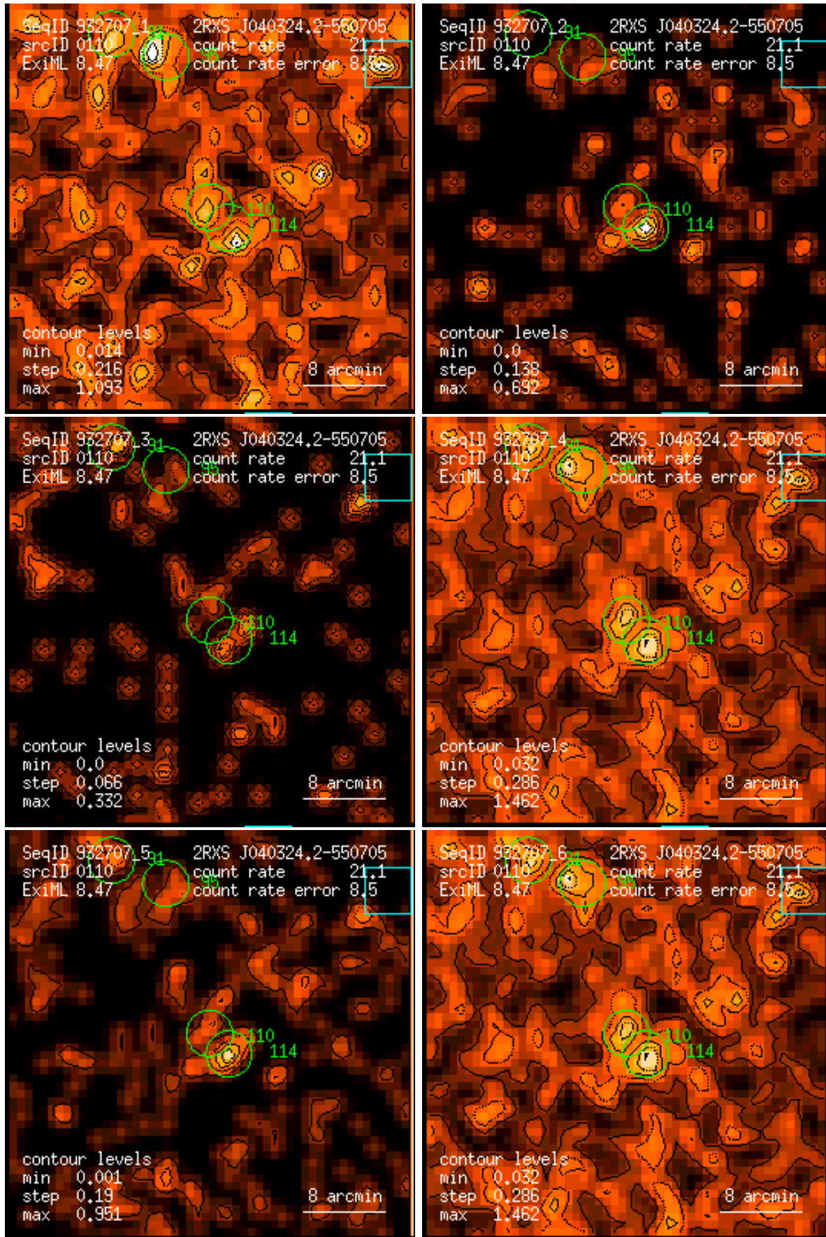
Figure 110: RASS 932707: detection 0110: band rate images, Gaussian filter: (1) PSPC channels 11 – 41, (2) 52 – 90, (3) 91 – 201, (4) 11 – 235, (5) 52 – 201, (6) 11 – 201. Broad band rates in counts/ks. Band rate contour levels in counts/ks/arcmin 2 .
