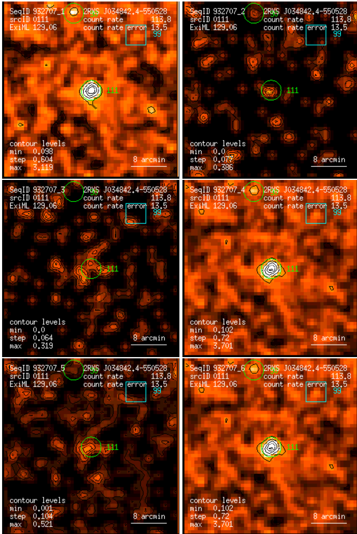
Figure 111: RASS 932707: detection 0111: band rate images, Gaussian filter: (1) PSPC channels 11 – 41, (2) 52 – 90, (3) 91 – 201, (4) 11 – 235, (5) 52 – 201, (6) 11 – 201. Broad band rates in counts/ks. Band rate contour levels in counts/ks/arcmin 2 .
