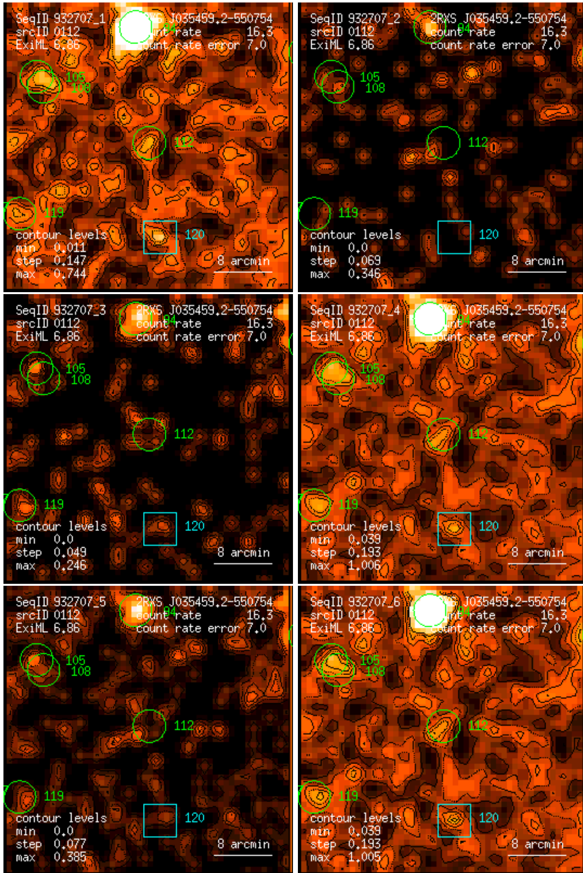
Figure 112: RASS 932707: detection 0112: band rate images, Gaussian filter: (1) PSPC channels 11 – 41, (2) 52 – 90, (3) 91 – 201, (4) 11 – 235, (5) 52 – 201, (6) 11 – 201. Broad band rates in counts/ks. Band rate contour levels in counts/ks/arcmin 2 .
