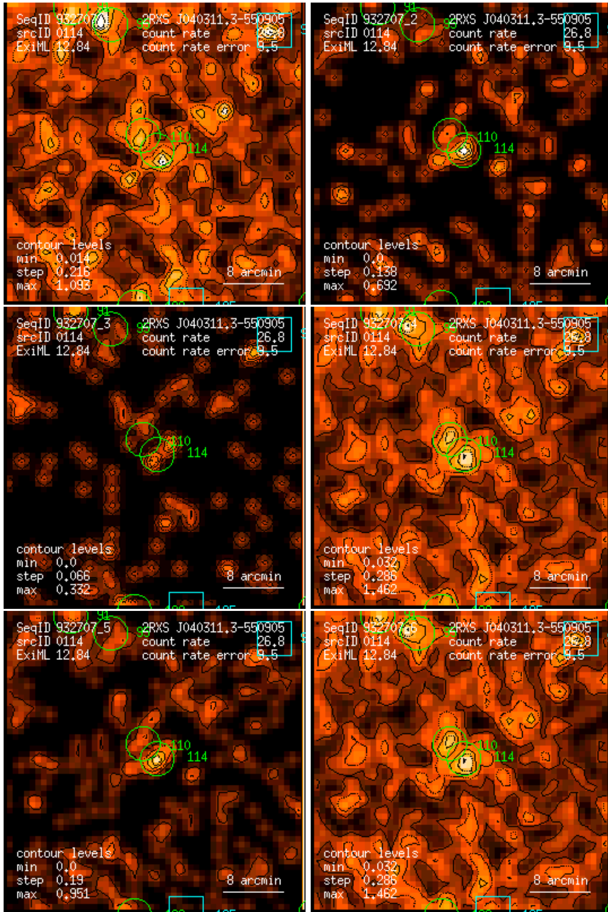
Figure 114: RASS 932707: detection 0114: band rate images, Gaussian filter: (1) PSPC channels 11 – 41, (2) 52 – 90, (3) 91 – 201, (4) 11 – 235, (5) 52 – 201, (6) 11 – 201. Broad band rates in counts/ks. Band rate contour levels in counts/ks/arcmin 2 .
