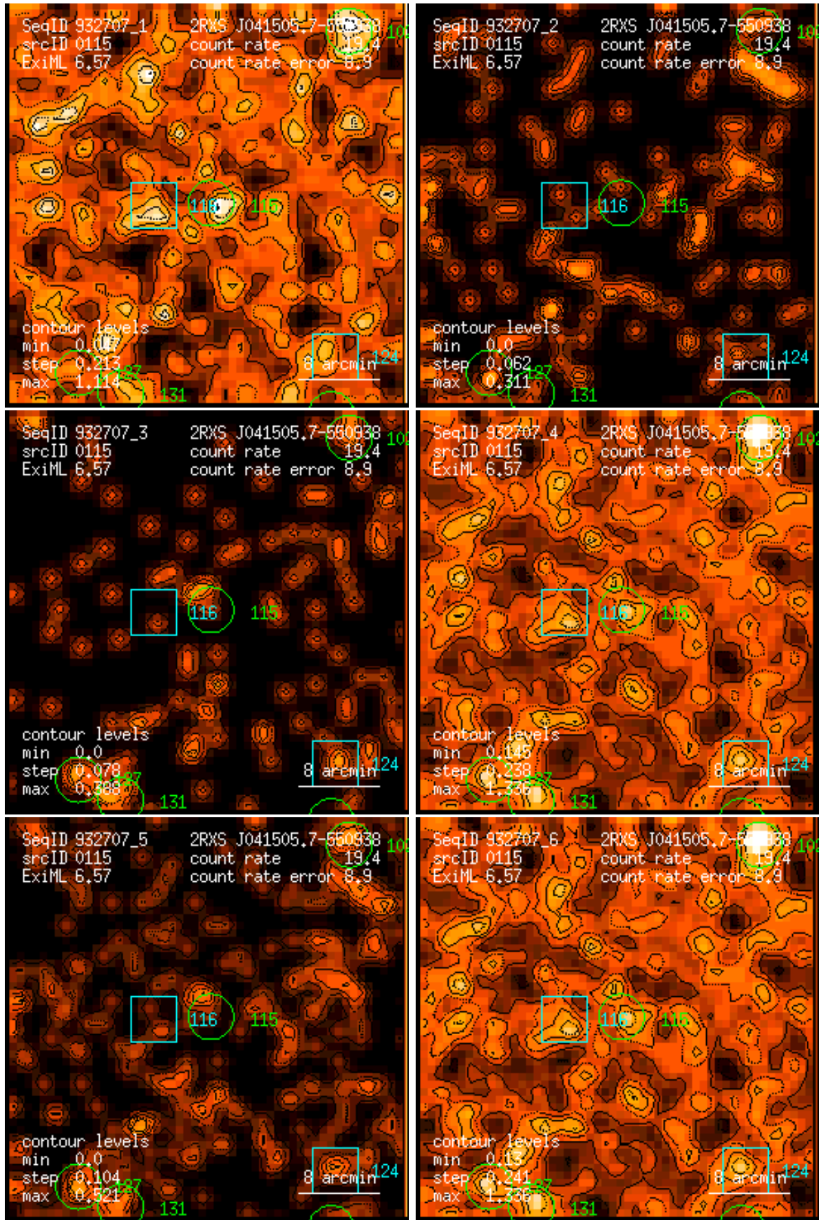
Figure 115: RASS 932707: detection 0115: band rate images, Gaussian filter: (1) PSPC channels 11 – 41, (2) 52 – 90, (3) 91 – 201, (4) 11 – 235, (5) 52 – 201, (6) 11 – 201. Broad band rates in counts/ks. Band rate contour levels in counts/ks/arcmin 2 .
