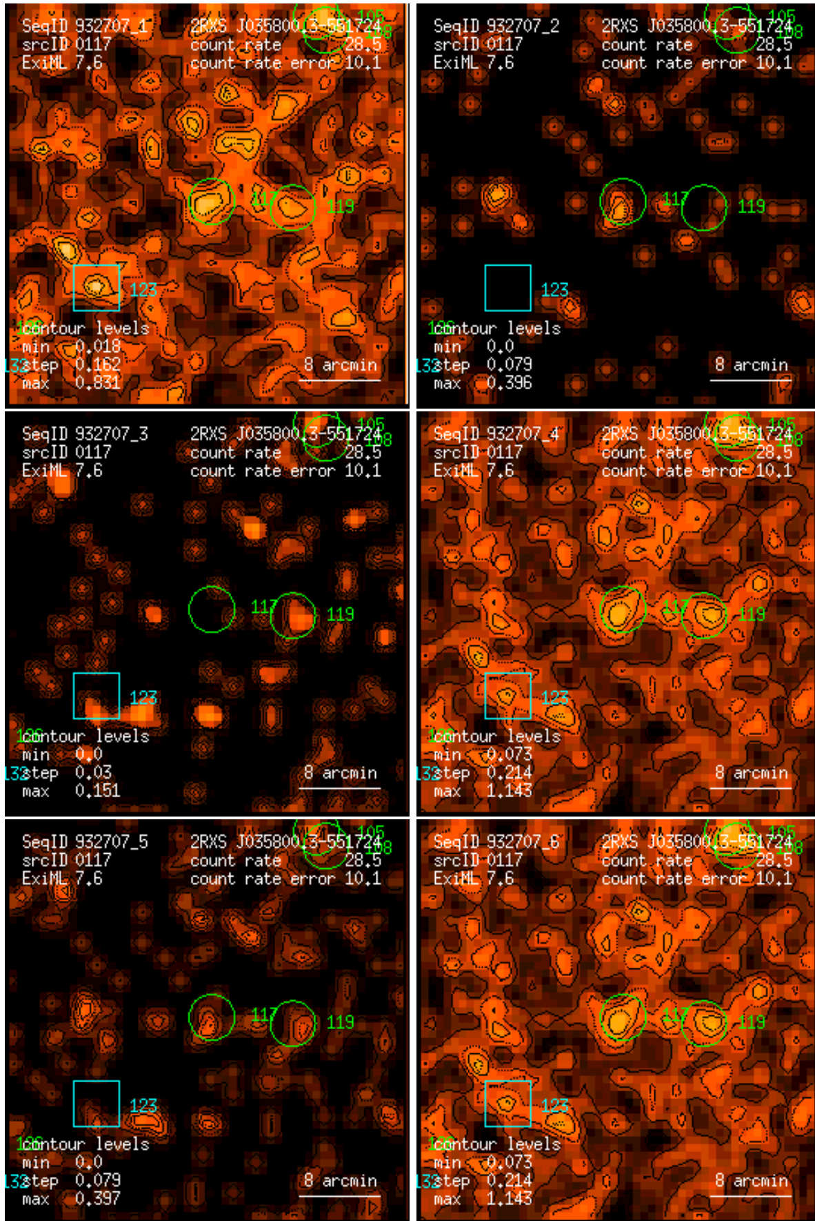
Figure 117: RASS 932707: detection 0117: band rate images, Gaussian filter: (1) PSPC channels 11 – 41, (2) 52 – 90, (3) 91 – 201, (4) 11 – 235, (5) 52 – 201, (6) 11 – 201. Broad band rates in counts/ks. Band rate contour levels in counts/ks/arcmin 2 .
