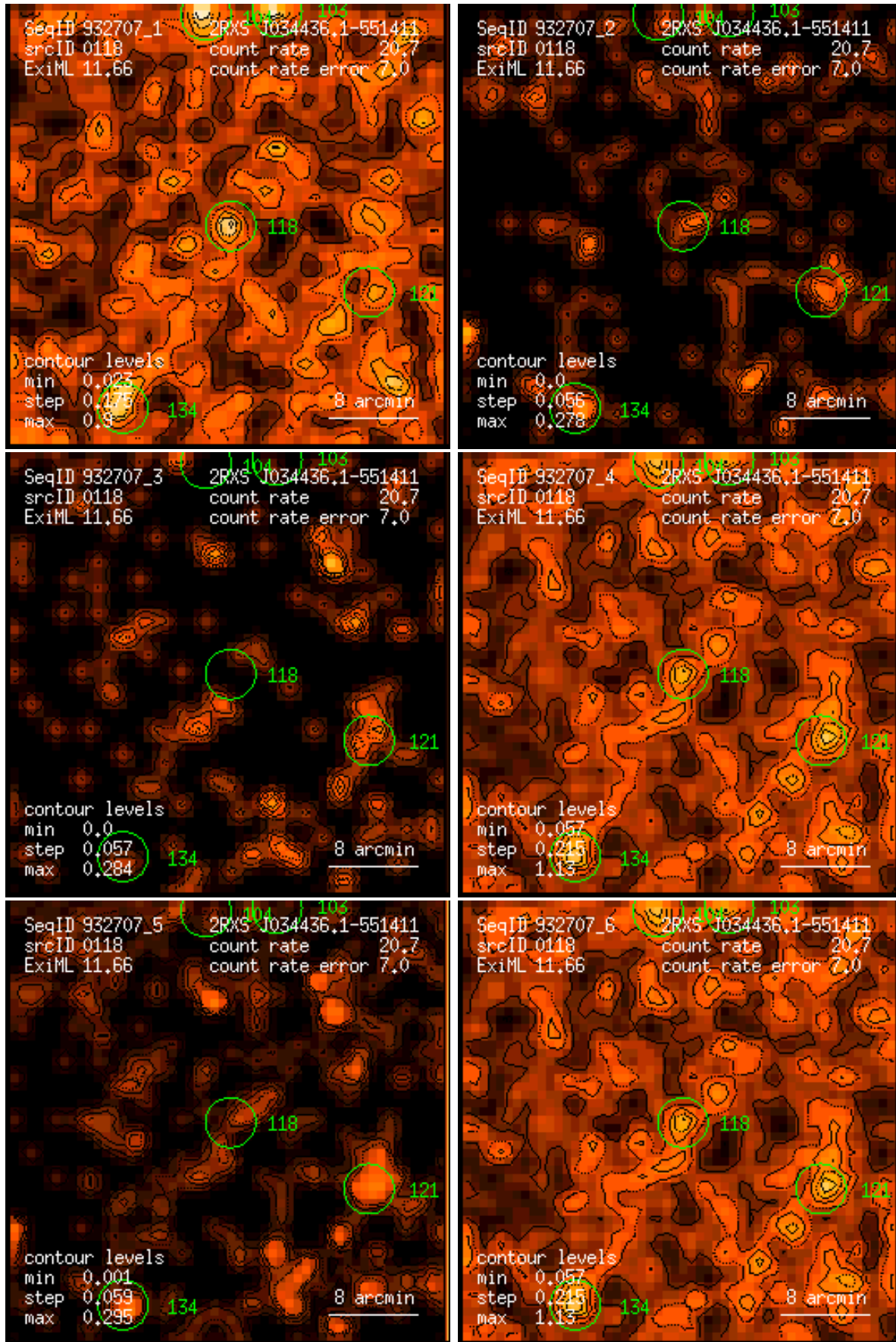
Figure 118: RASS 932707: detection 0118: band rate images, Gaussian filter: (1) PSPC channels 11 – 41, (2) 52 – 90, (3) 91 – 201, (4) 11 – 235, (5) 52 – 201, (6) 11 – 201. Broad band rates in counts/ks. Band rate contour levels in counts/ks/arcmin 2 .
