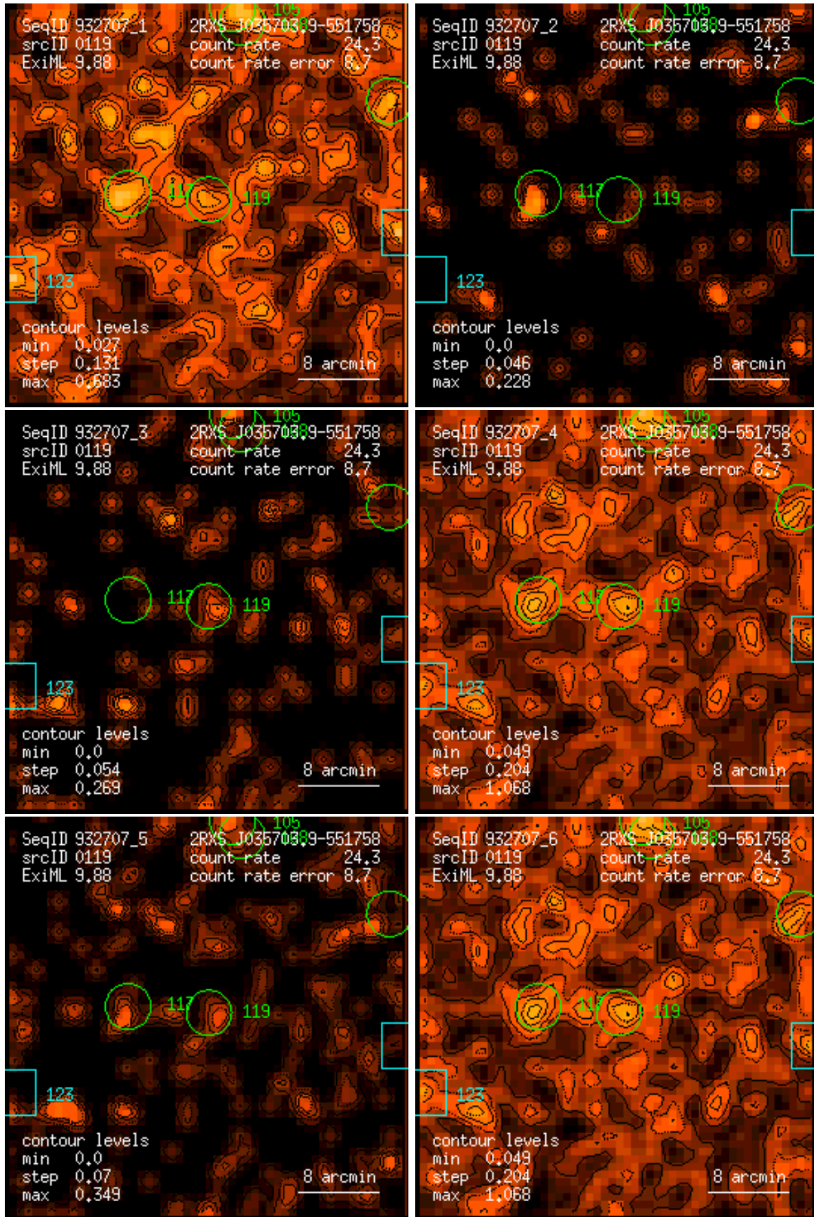
Figure 119: RASS 932707: detection 0119: band rate images, Gaussian filter: (1) PSPC channels 11 – 41, (2) 52 – 90, (3) 91 – 201, (4) 11 – 235, (5) 52 – 201, (6) 11 – 201. Broad band rates in counts/ks. Band rate contour levels in counts/ks/arcmin 2 .
