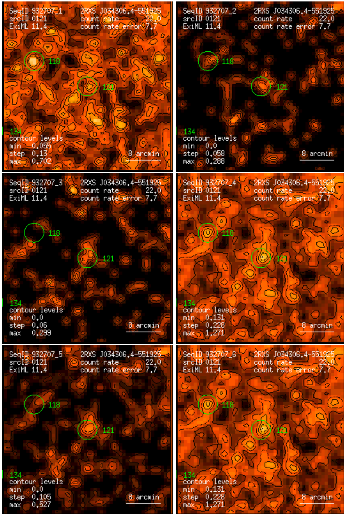
Figure 121: RASS 932707: detection 0121: band rate images, Gaussian filter: (1) PSPC channels 11 – 41, (2) 52 – 90, (3) 91 – 201, (4) 11 – 235, (5) 52 – 201, (6) 11 – 201. Broad band rates in counts/ks. Band rate contour levels in counts/ks/arcmin 2 .
