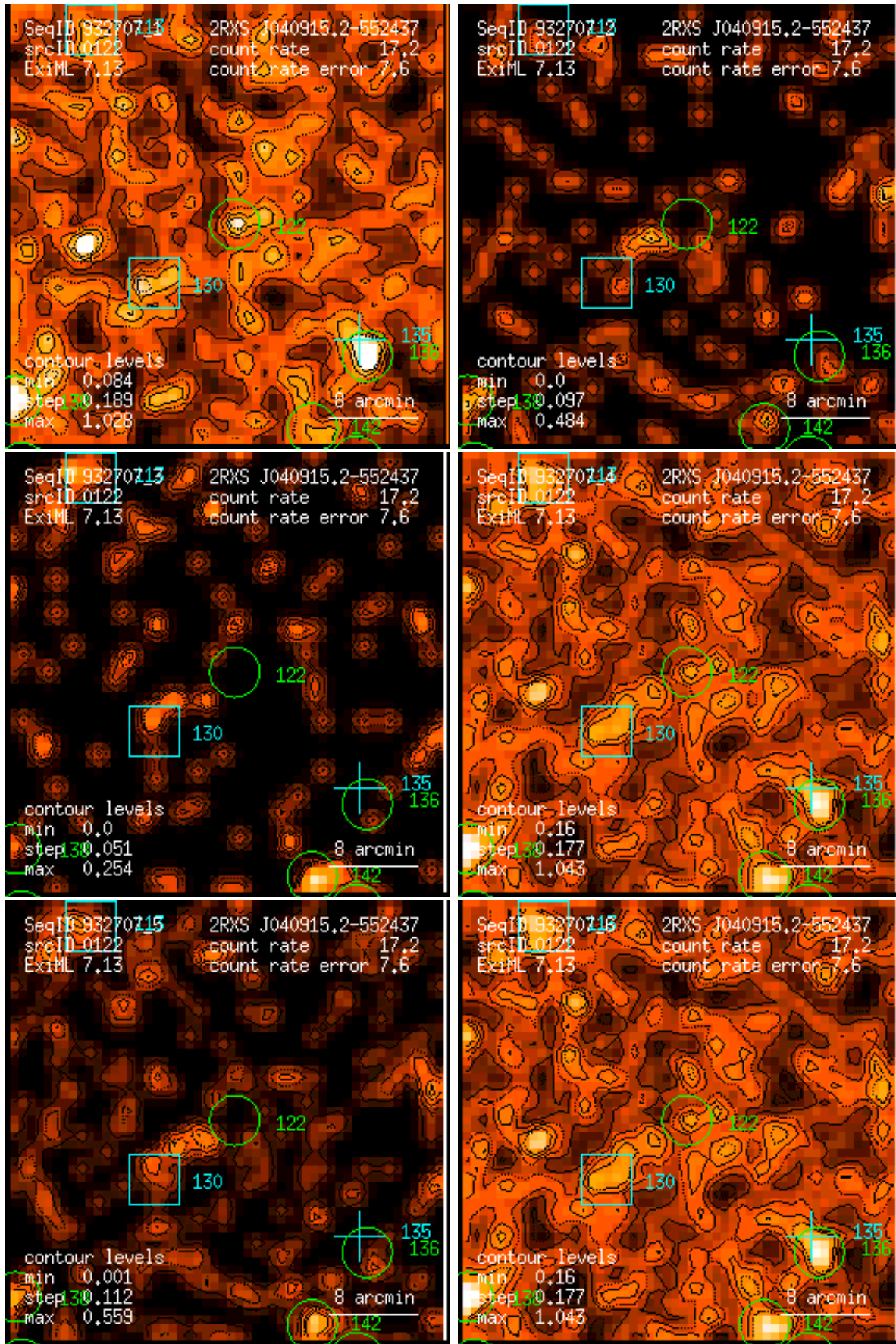
Figure 122: RASS 932707: detection 0122: band rate images, Gaussian filter: (1) PSPC channels 11 – 41, (2) 52 – 90, (3) 91 – 201, (4) 11 – 235, (5) 52 – 201, (6) 11 – 201. Broad band rates in counts/ks. Band rate contour levels in counts/ks/arcmin 2 .
